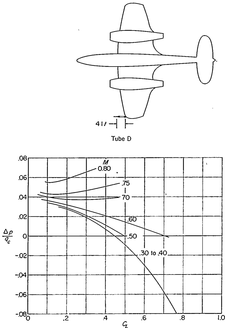
FIGURE 32.—Variation of static-pressure error with lift coefficient for a wing-tip installation on an unswept-wing airplane (ref. 27).
