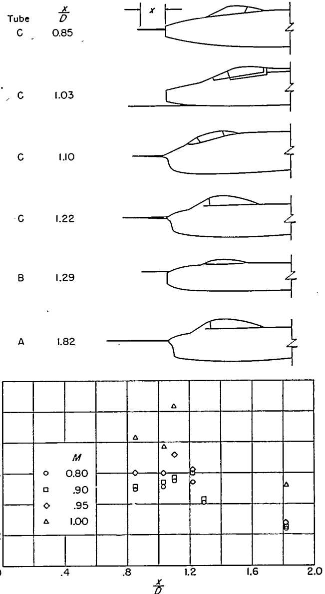
FIGURE 27.—Static-pressure errors ahead of six airplane fuselages with nose inlets.
