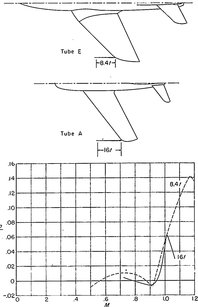
FIGURE 33.—Calibration in level flight of wing-tip installations on two swept-wing airplanes (refs. 28 and 29).
