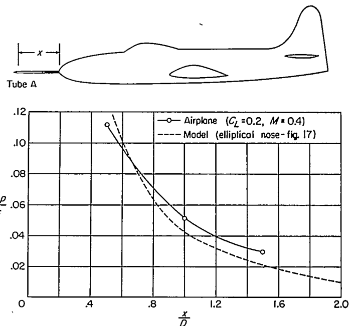
FIGURE 18.—Static-pressure errors at three distances ahead of an airplane fuselage with an elliptical nose shape (ref. 22).
