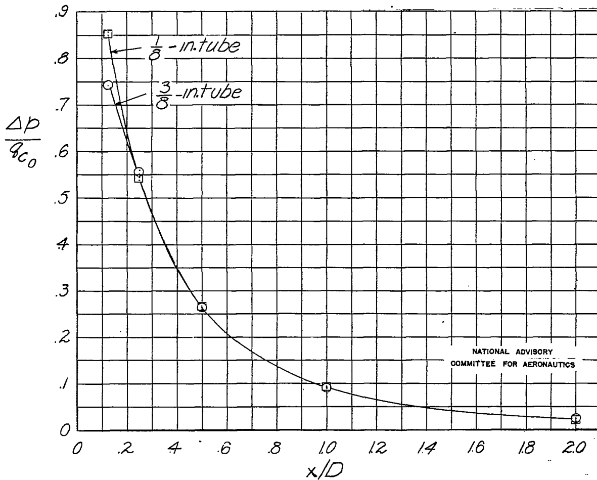
Figure 8.- Effect of tube diameter on the error in static pressure caused by fuselage interference. Circular-nose fuselage; \alpha = 0^\circ ; q_c = 65 pounds per square foot.
