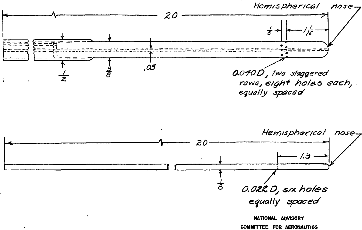
Figure 3.- Details of tubes used in tests. All dimensions are in inches.
