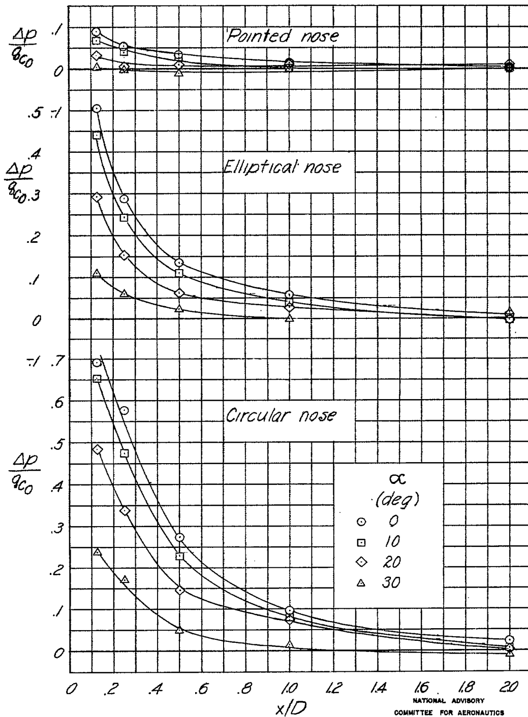
Figure 5.- Effect of angle of attack on the error in static pressure caused by fuselage interference. q_c = 40 pounds per square foot.
