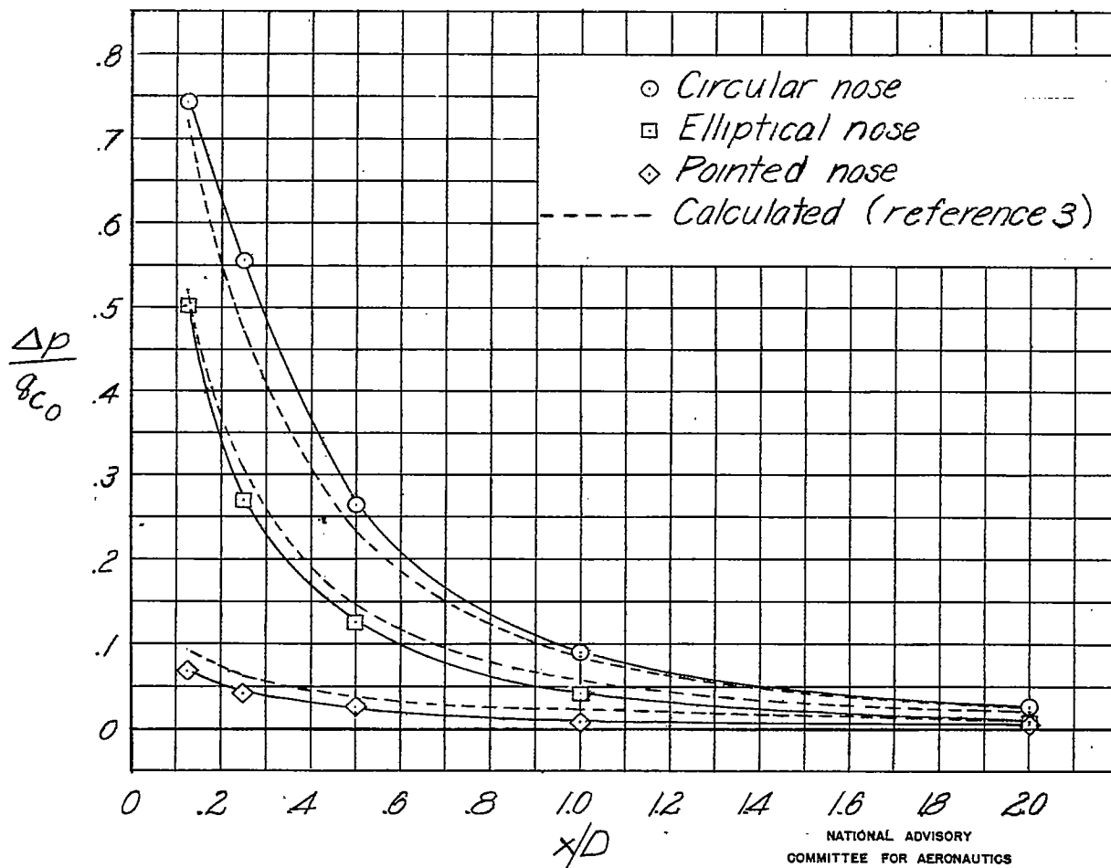
Figure 4.- Effect of fuselage nose shape on the error in static pressure caused by fuselage interference. \alpha = 0^\circ ; q_c = 65 pounds per square foot.
