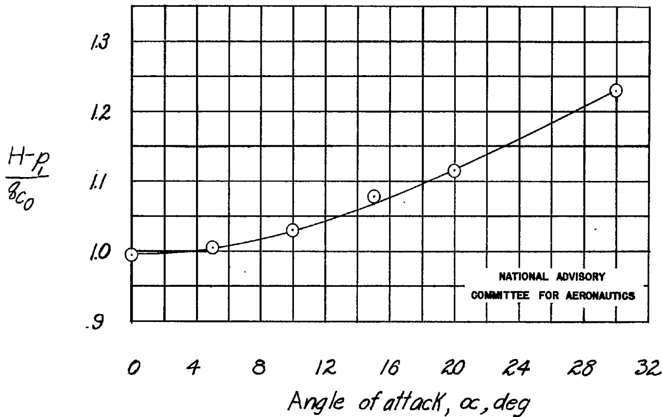
Figure 6.- Calibration of static-pressure error of the \frac{3}{8} -inch-diameter pitot-static tube. q_c = 40 pounds per square foot.
