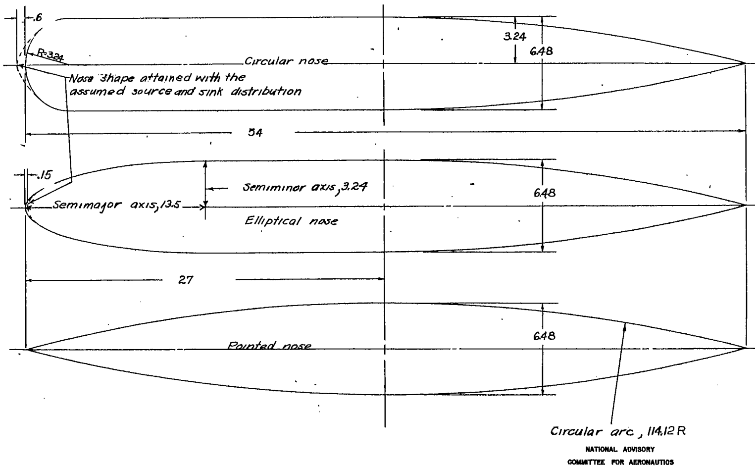
Figure 2.- Details of fuselages used in tests. All dimensions are in inches.
