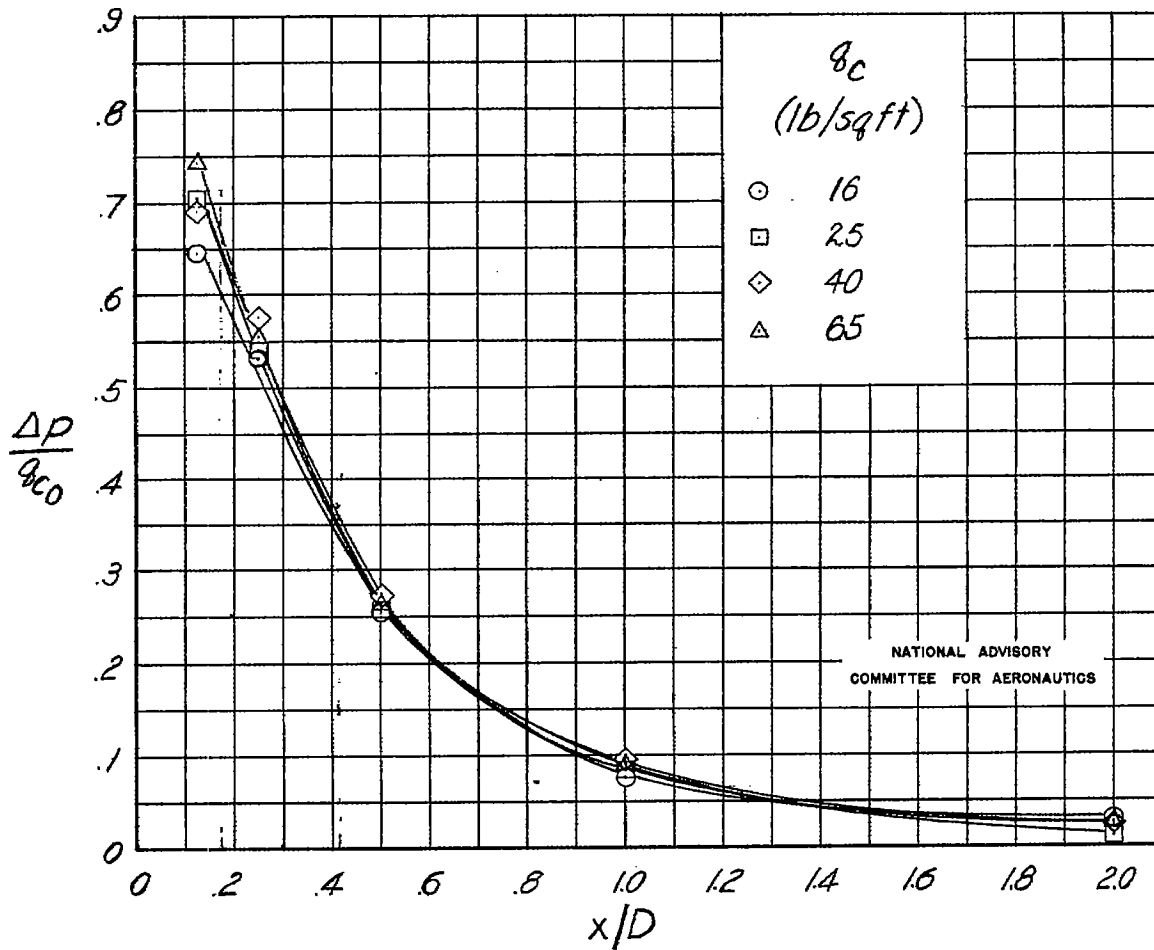
Figure 7.- Effect of free-stream impact pressure on the error in static pressure caused by fuselage interference. Circular-nose fuselage; \alpha = 0^\circ .
