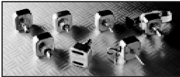
Photo 2 —These incremental rotary optical encoders provide quadrature digital output. Encoder use is increasing as more transducers are being connected directly to digital processing systems.
