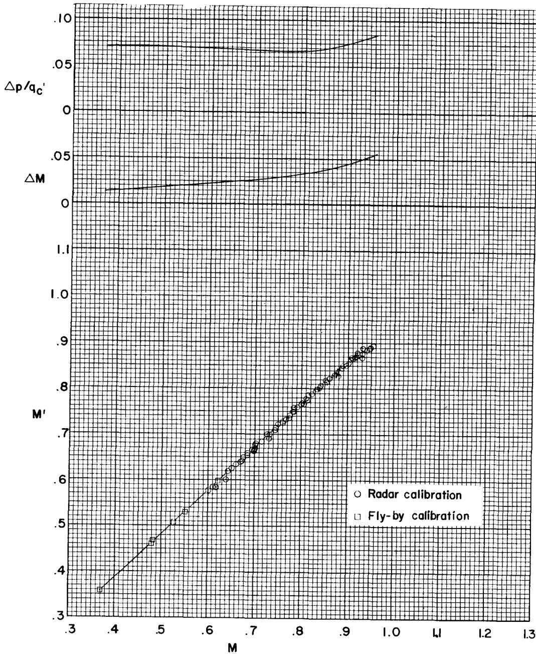
Figure 10.- Static-pressure errors for airplane H.
