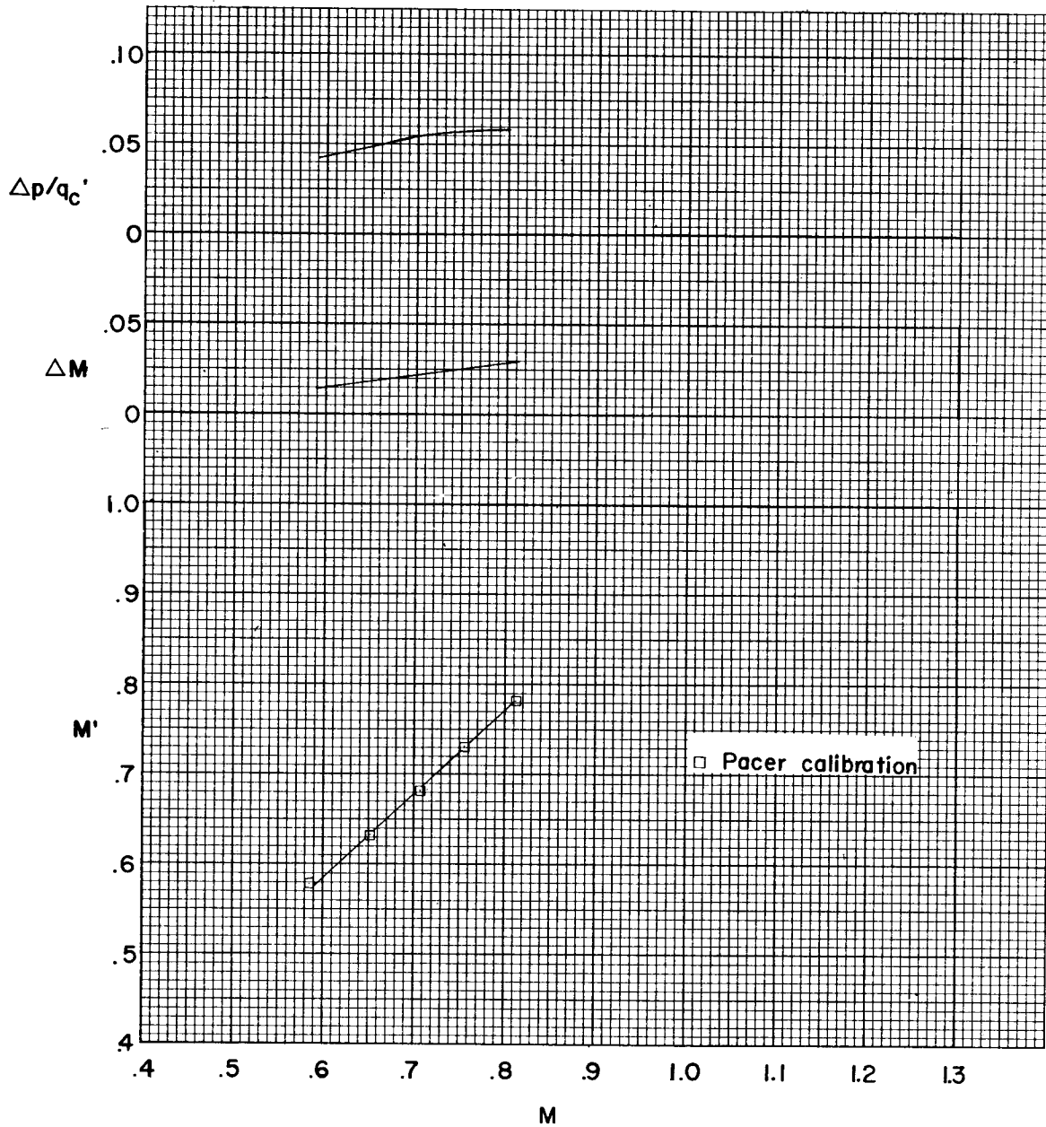
Figure 16.- Static-pressure errors for airplane Q.
