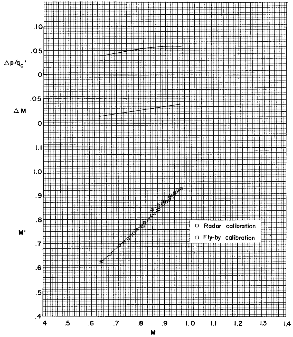
Figure 5.- Static-pressure errors for airplane C.
