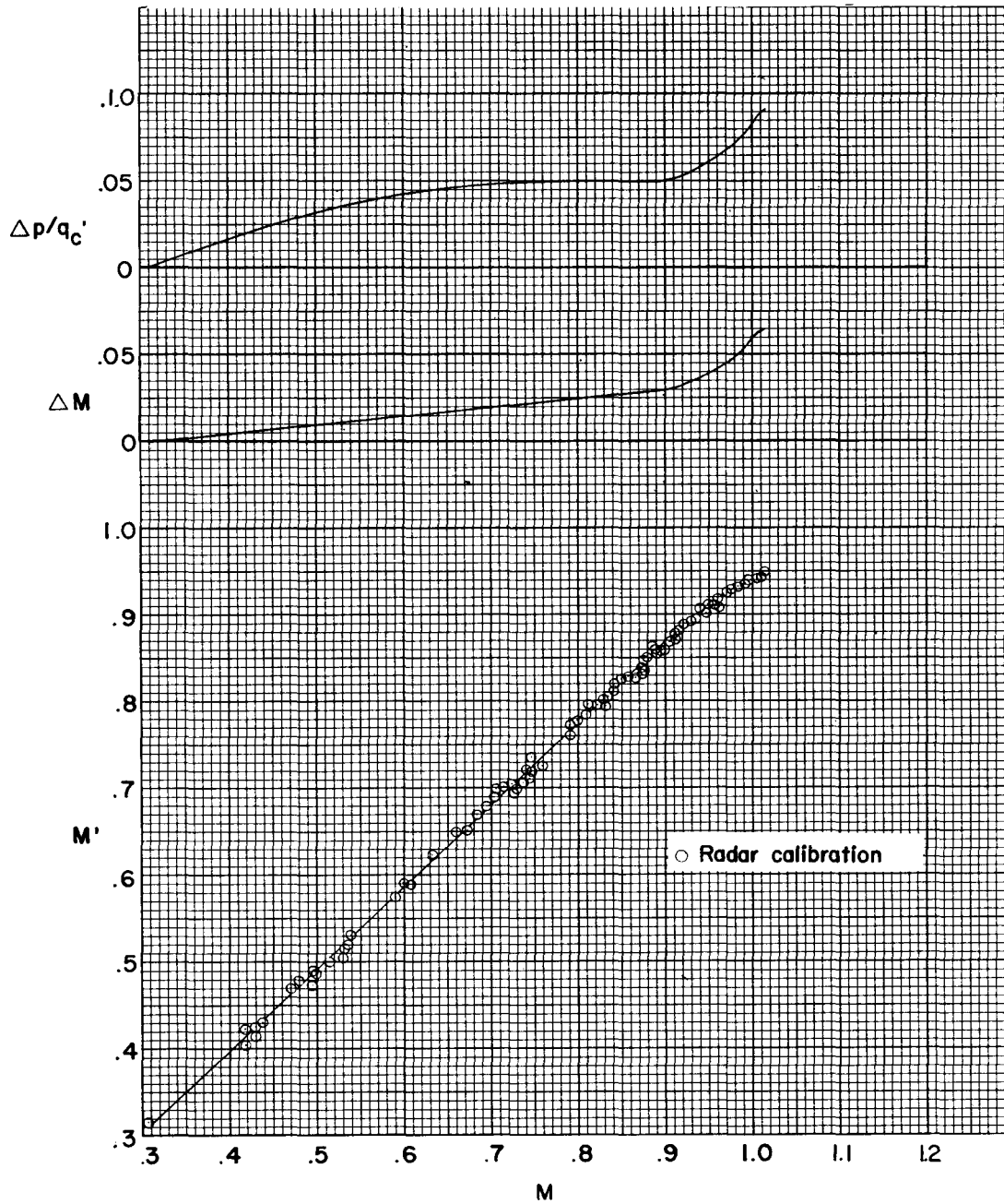
Figure 8.- Static-pressure errors for airplane F.
