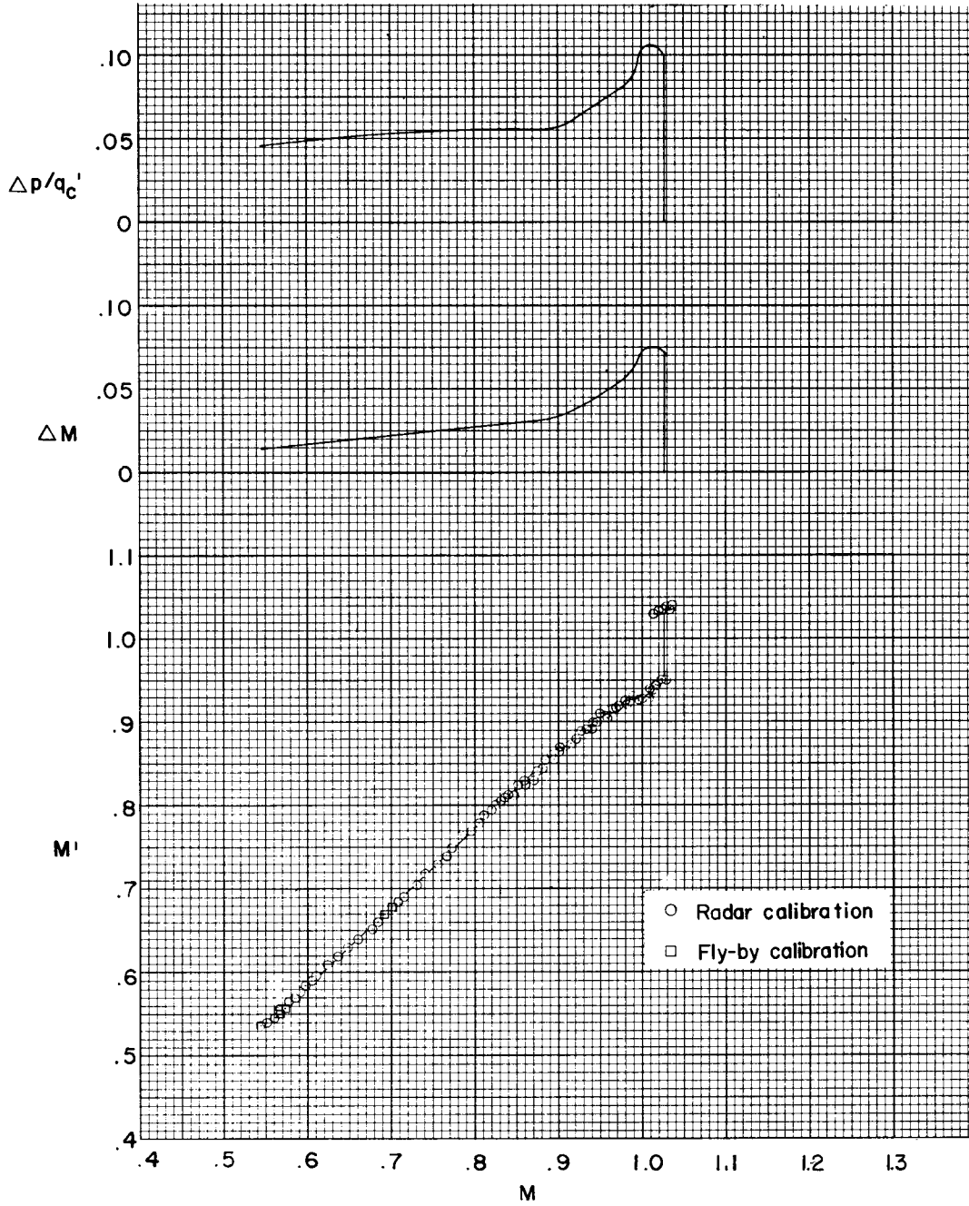
Figure 6.- Static-pressure errors for airplane D.
