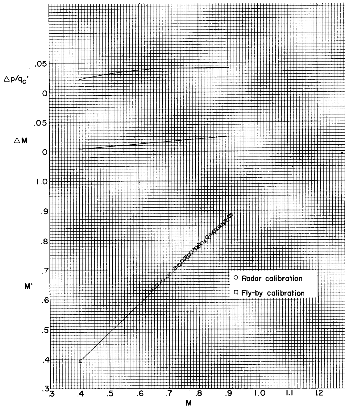
Figure 3.- Static-pressure errors for airplane A.
