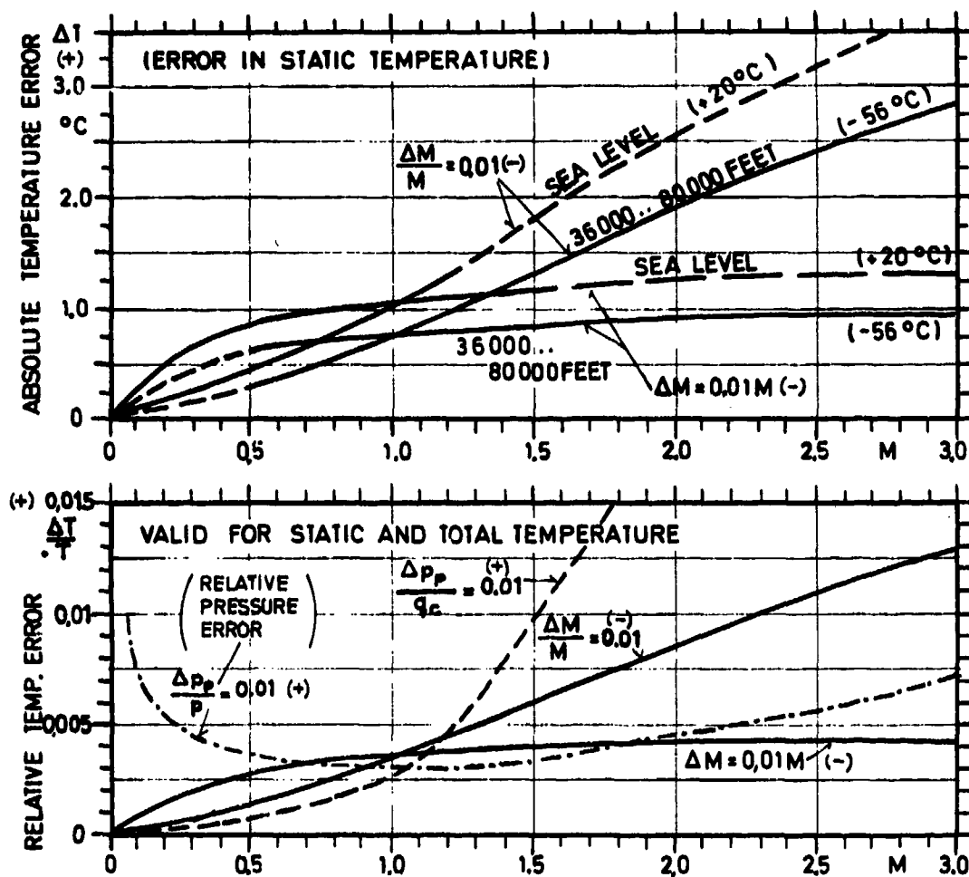
Fig.99 Absolute and relative error in static temperature vs. Mach number as functions of given values of absolute and relative errors in Mach number
