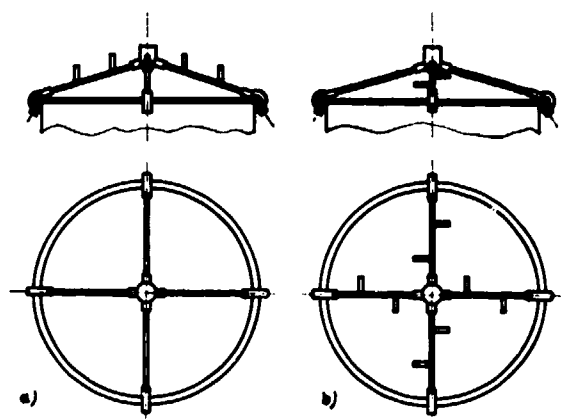
Fig. 66 Alternative mounts of TAT-sensors for CIT measurement in a vertical lift engine
