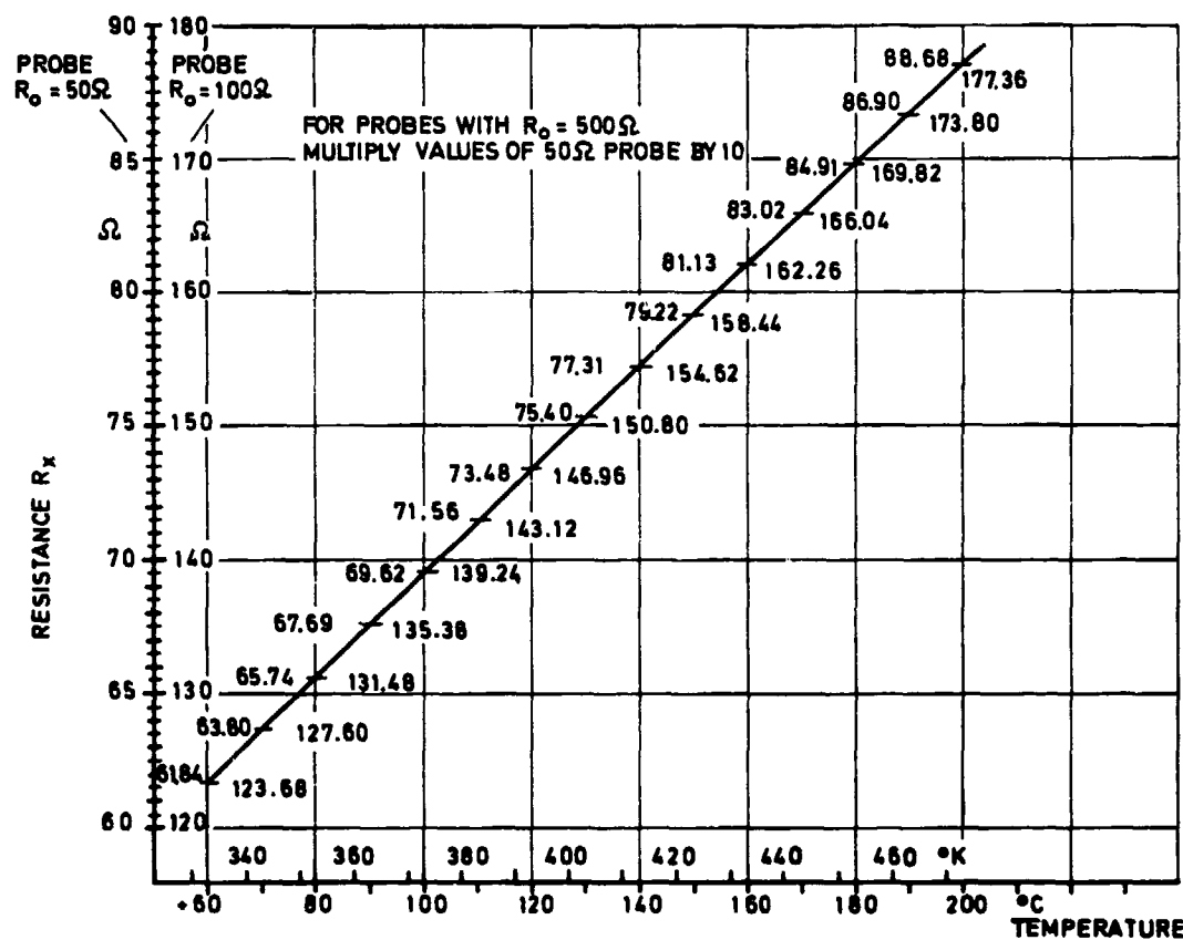
Fig.5(b) Cont., range +60 to +200^\circ\text{C} (platinum, MIL-P-25726).
