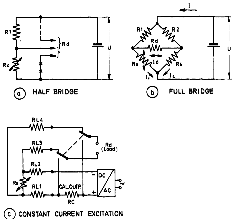
Fig.24 Typical bridge circuits
