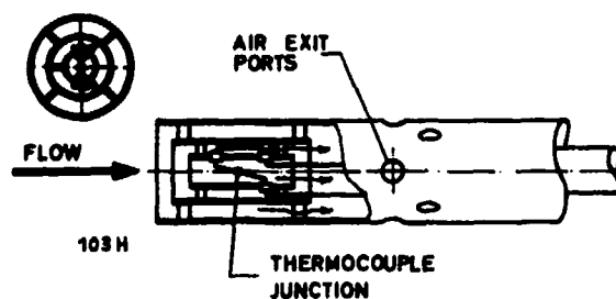
Fig. 40 Special TAT probe with thermocouple
