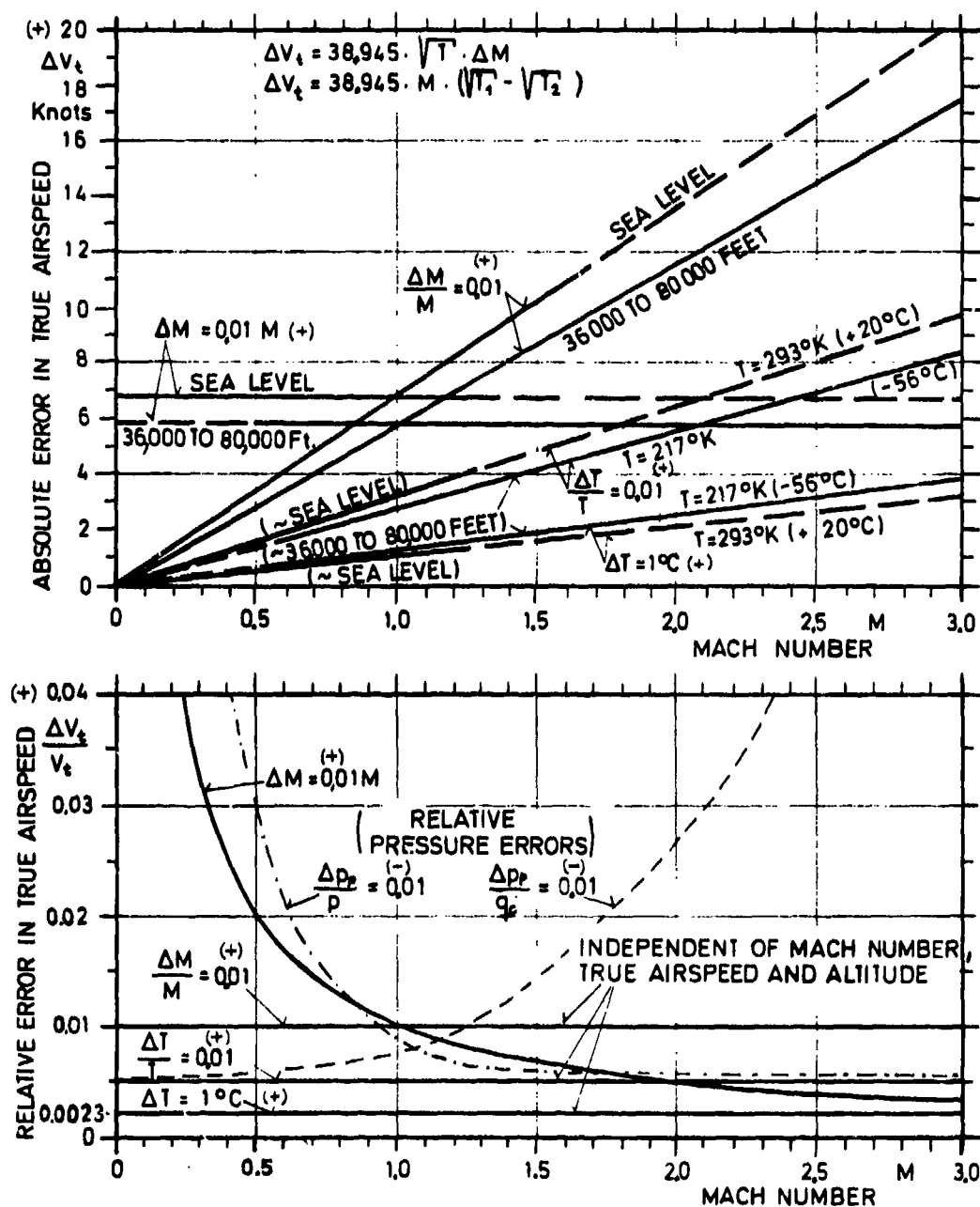
Fig.113 Absolute and relative error in the airspeed vs. Mach number as functions of given values of abs. and rel. errors in Mach number and static temperature
