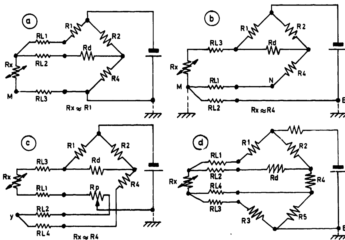
Fig.25 Compensation of lead-resistances
