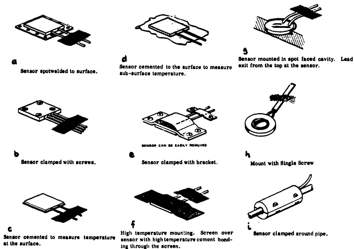
Fig.94 Installation of surface temperature sensors
