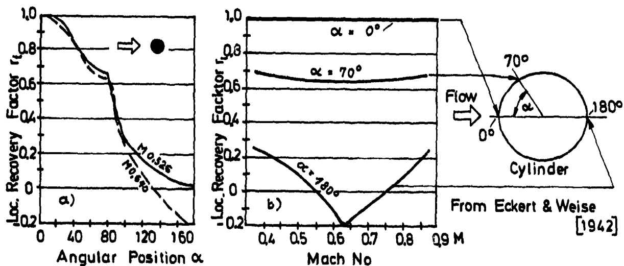
Fig.54 Distribution of local recovery factors around a cylinder in cross flow vs Mach number
