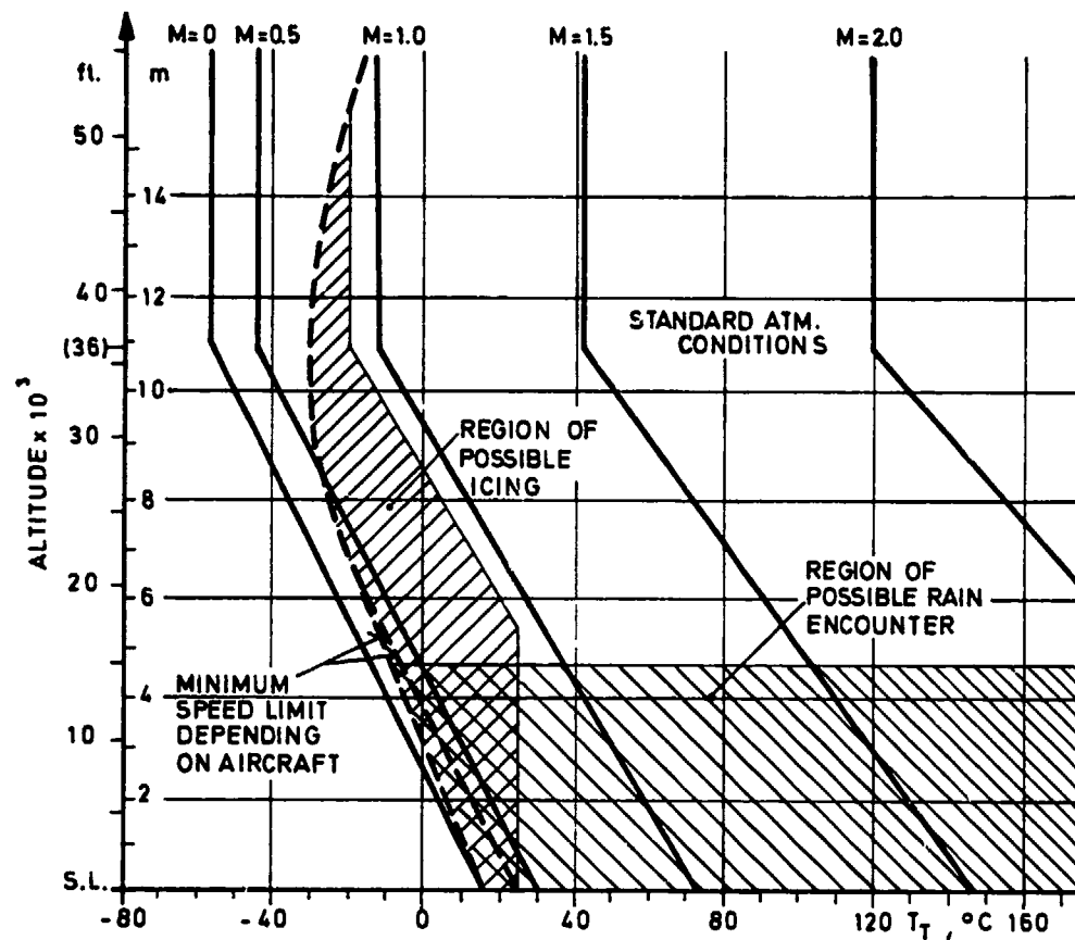
Fig.60 Total temperature as a function of altitude and Mach number
