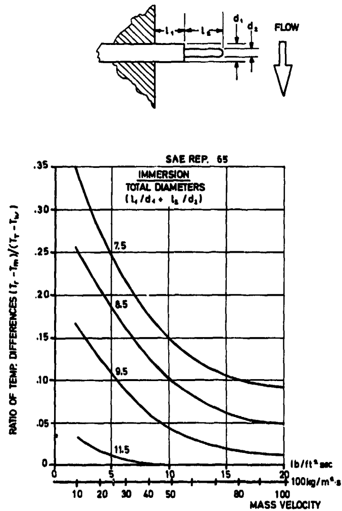
Fig.73 Conduction correction factor of EGT-probes vs. mass velocity
