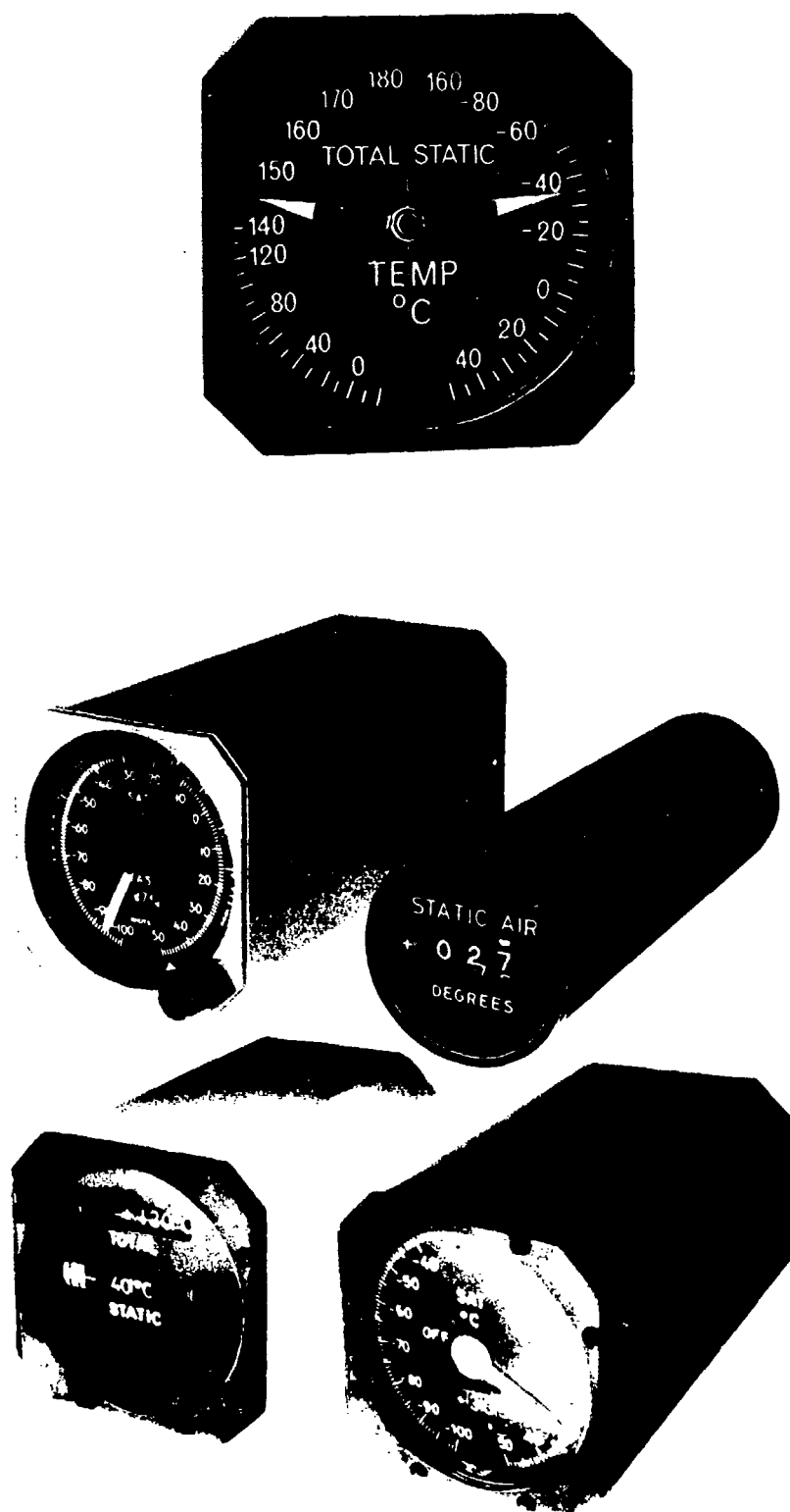
Fig.34 Different types of servoed indicators, single and combined versions
