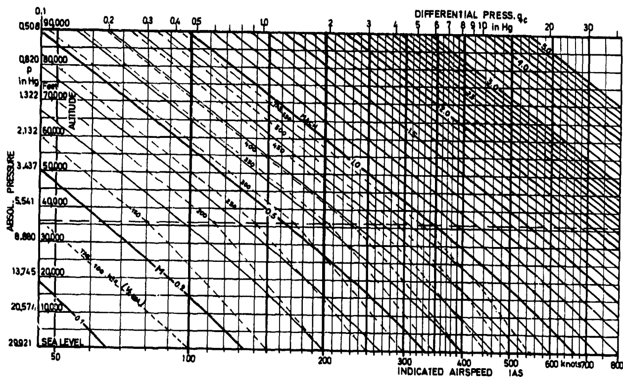
Fig.112 Mach number vs. indicated airspeed and pressure altitude
