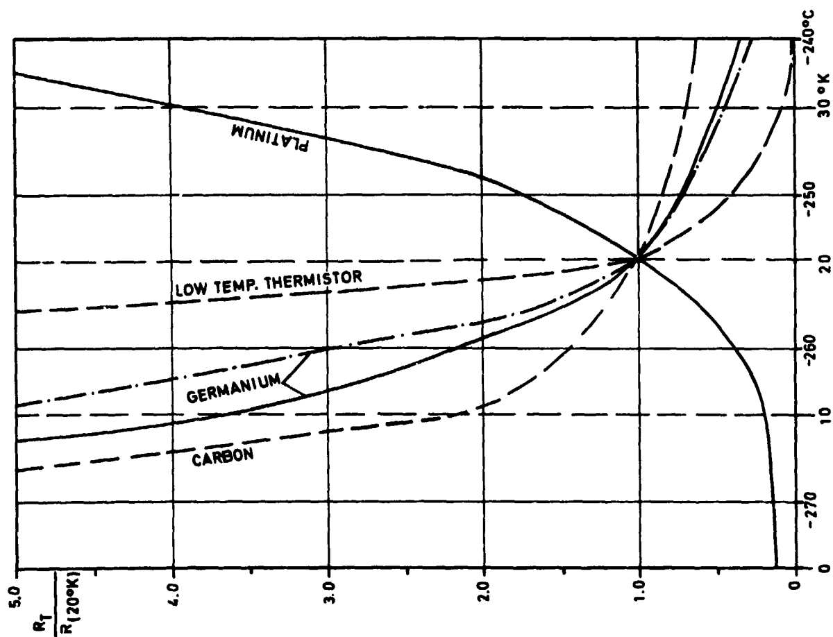
Fig. 8(a) Resistance-temperature relationship of low temperature sensors.
