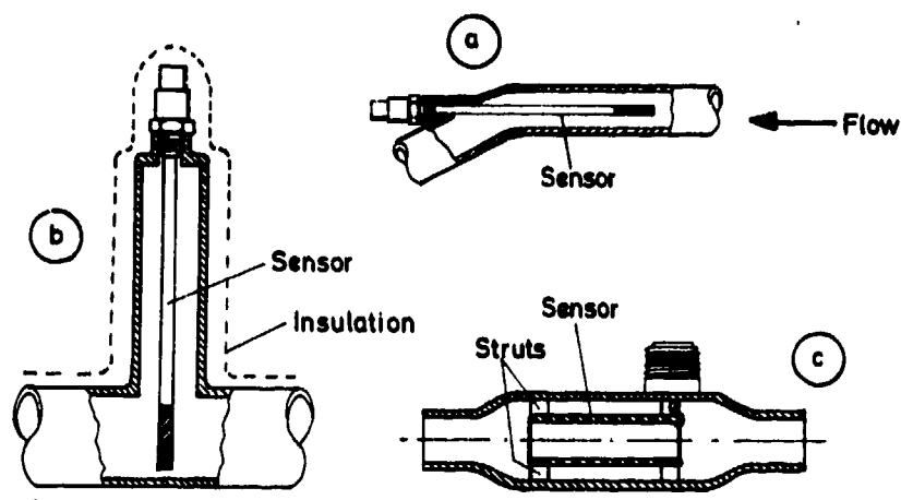
Fig.93 Typical probe installations in tubing
