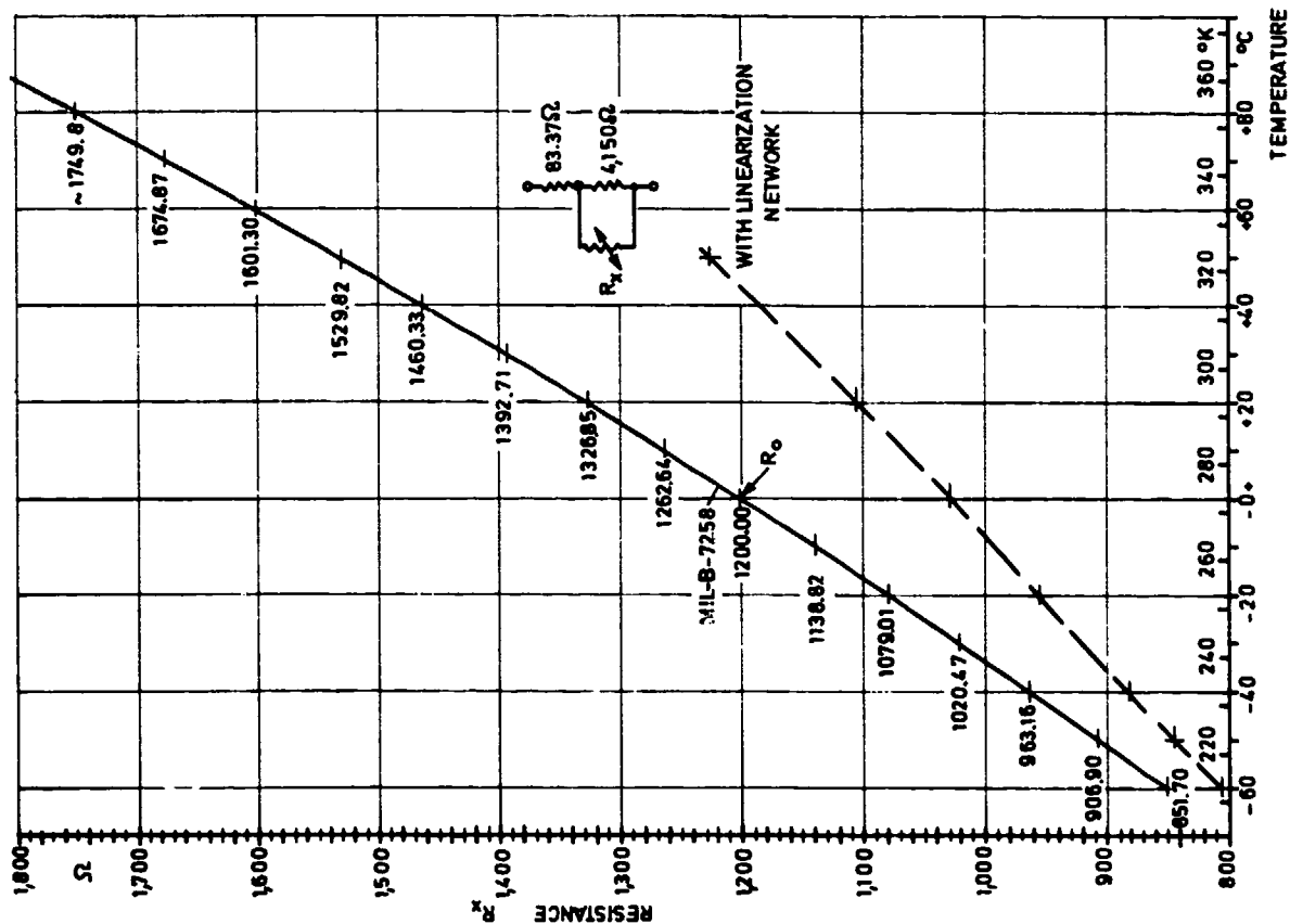
Fig. 6(a) Resistance-temperature relationship of nickel element MIL-B-7258
