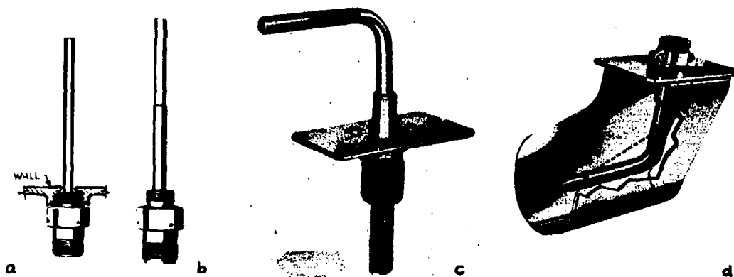
(a,b) for use in cross-flow (c) L-shaped probe for parallel-flow (d) ditto, with protecting shield
