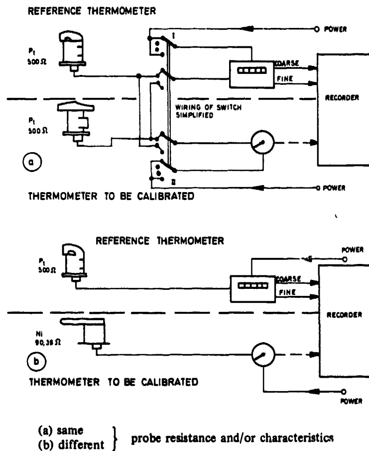
Fig.104 Connection of reference thermometer and thermometer to be calibrated
