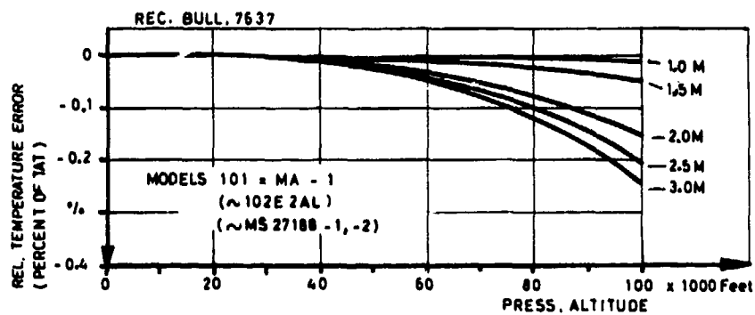
Fig.71 Typical radiation error of some TAT-probes
