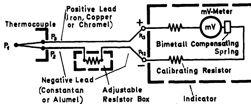
Fig.44 Wiring diagram -- simple thermocouple thermometer
