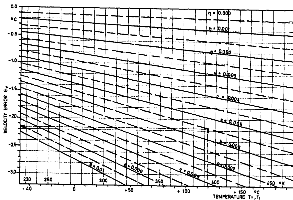
Fig.111 Velocity error E_v as a function of recovery error \eta and total temperature T_t \approx recovery temperature T_r
