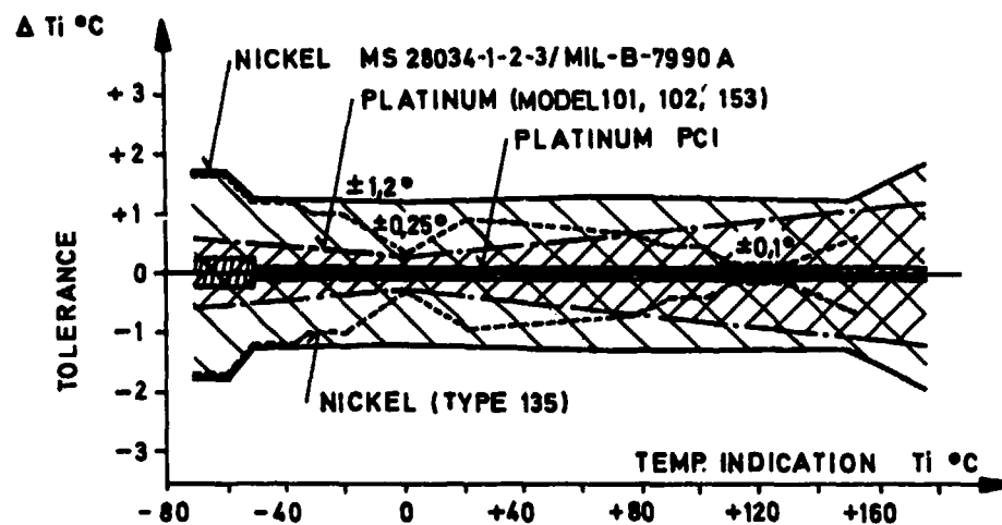
Fig. 87(a) Typical tolerances (calibration error) of resistance probes. Note: PCI = precision calibration interchangeability
