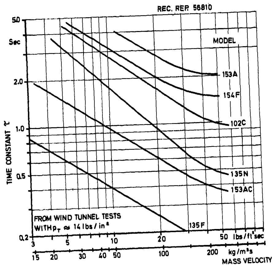
Fig.81 Typical time constants of some CIT-probes vs. mass velocity
