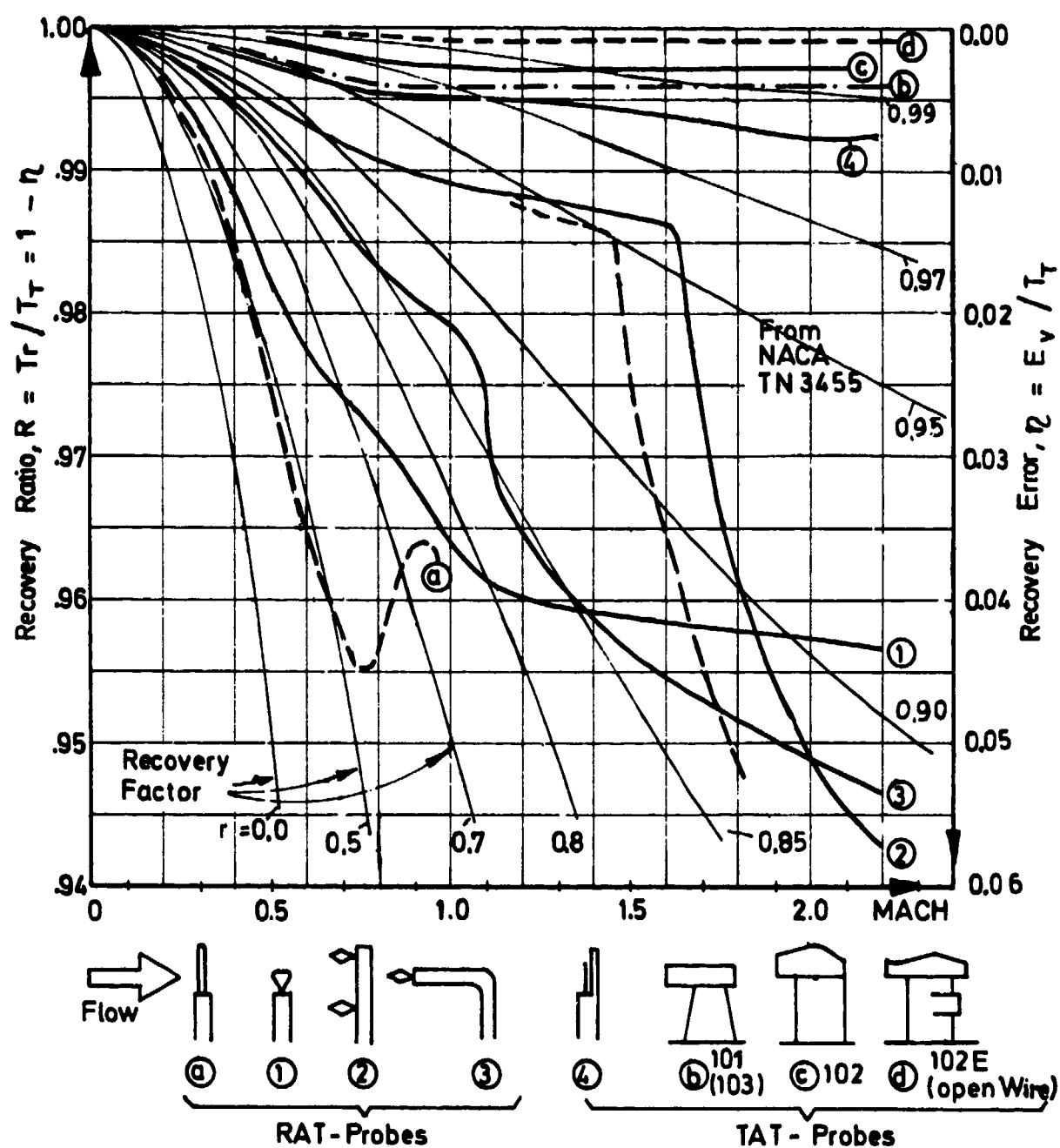
Fig. 67 Recovery ratio, recovery factor and recovery error of different probes
