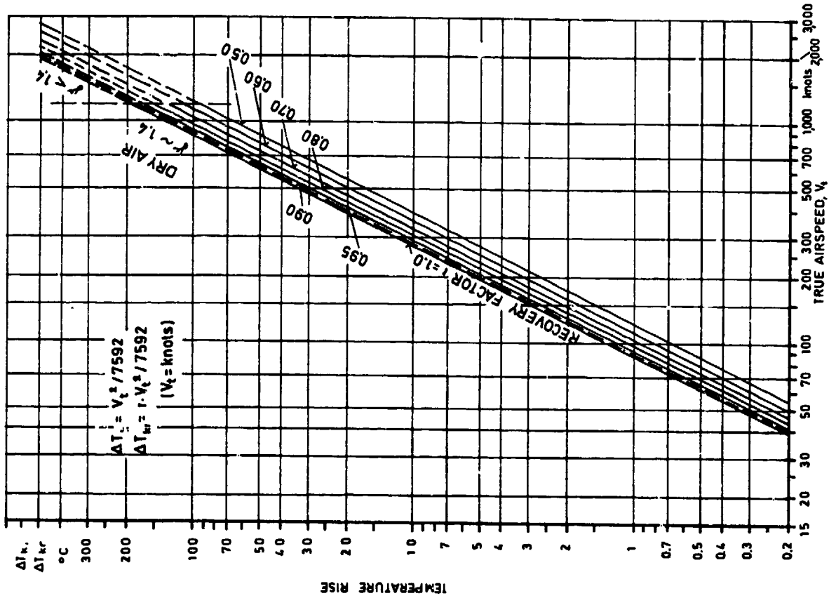
Fig. 58 Kinetic temperature rise for various recovery factors vs true airspeed
