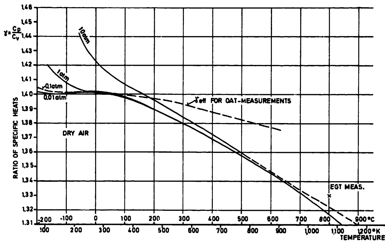
Fig.62(b) Variation of \gamma vs temperature
