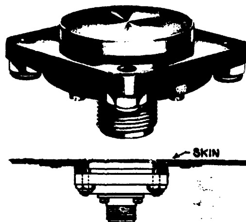
Fig. 14 Flush-bulb
