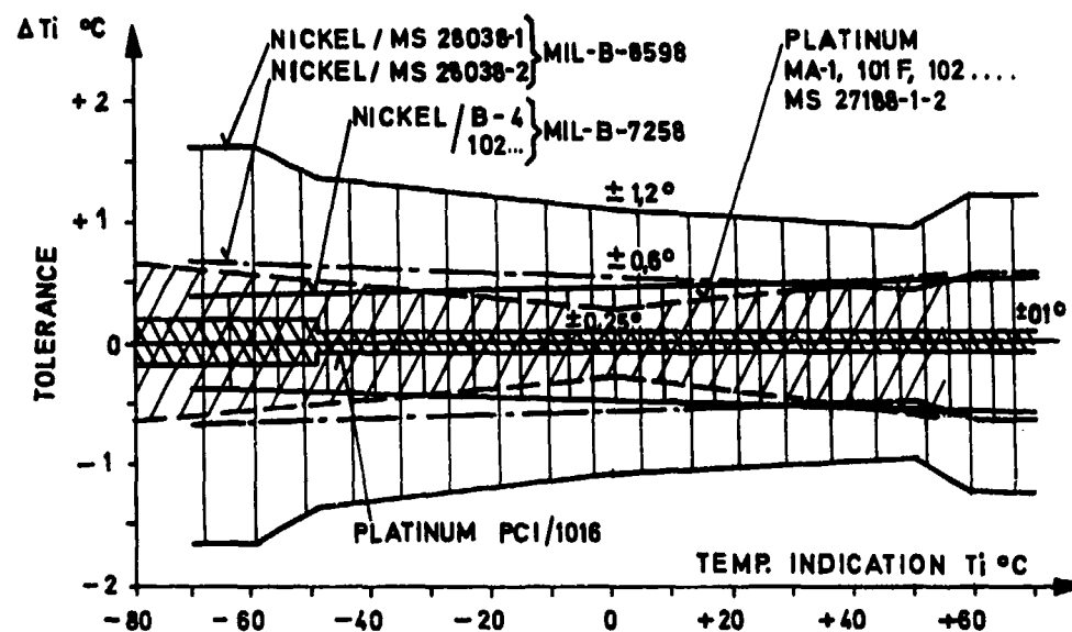
Fig. 87(b) Typical tolerances (calibration error) of resistance probes
