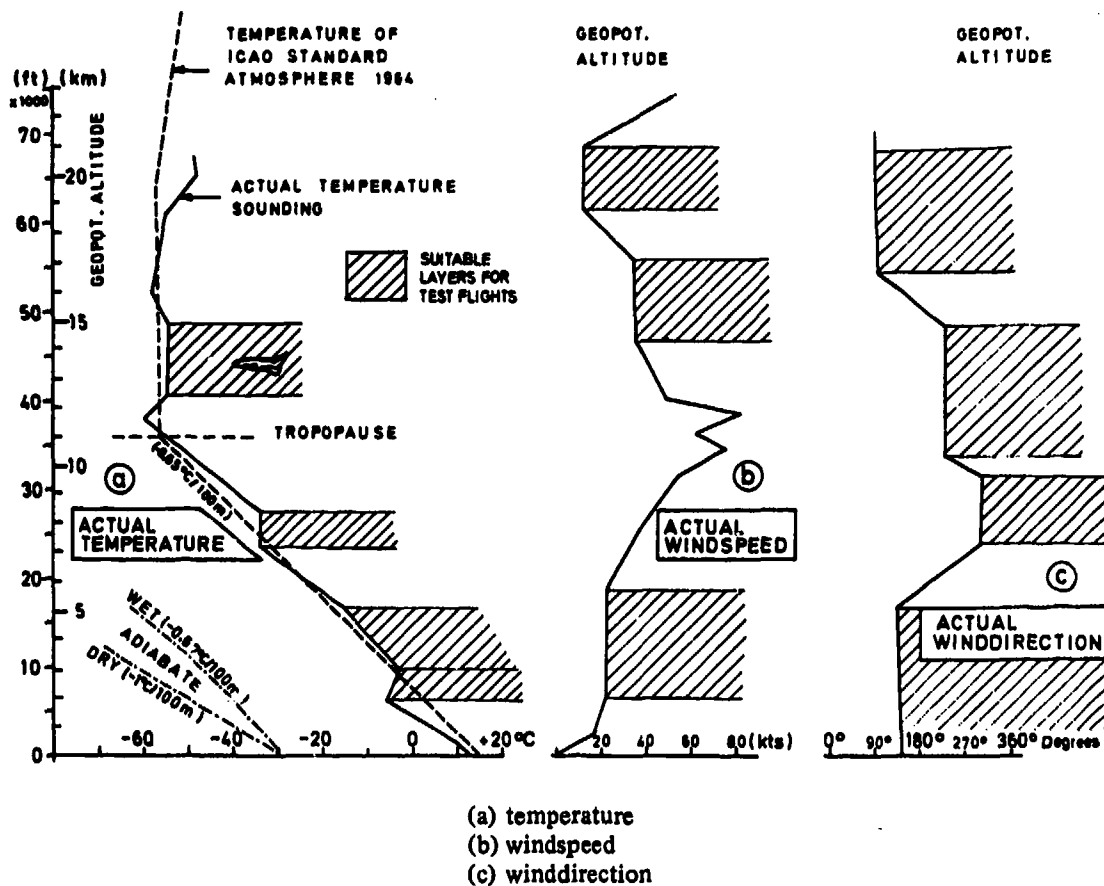
Fig.103 Suitable meteorological conditions for temperature calibration flights
