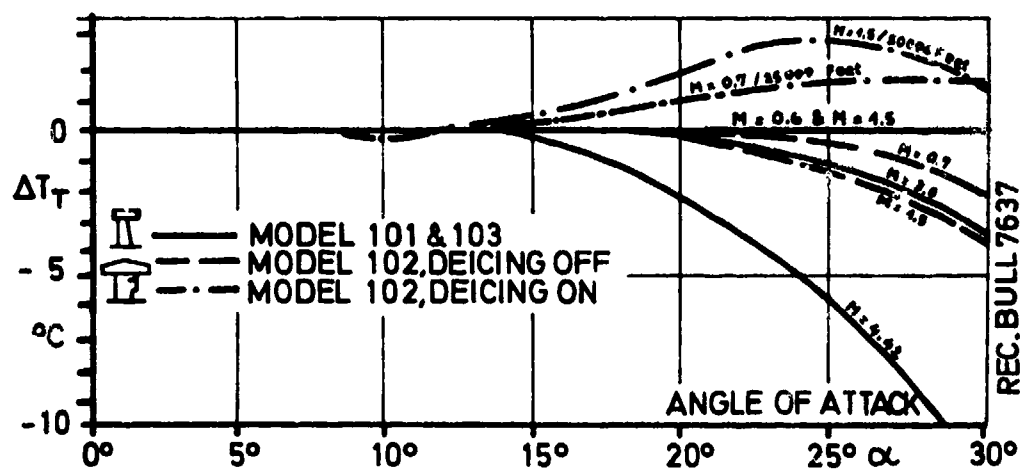
Fig.64 Attitude error of some TAT-probes
