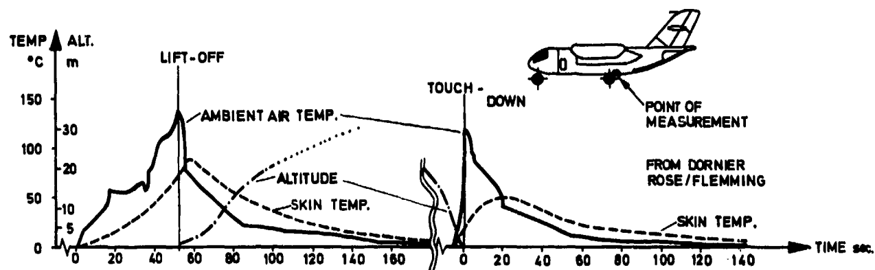
Fig.98(a) Skin temperature at vertical take-off and landing
