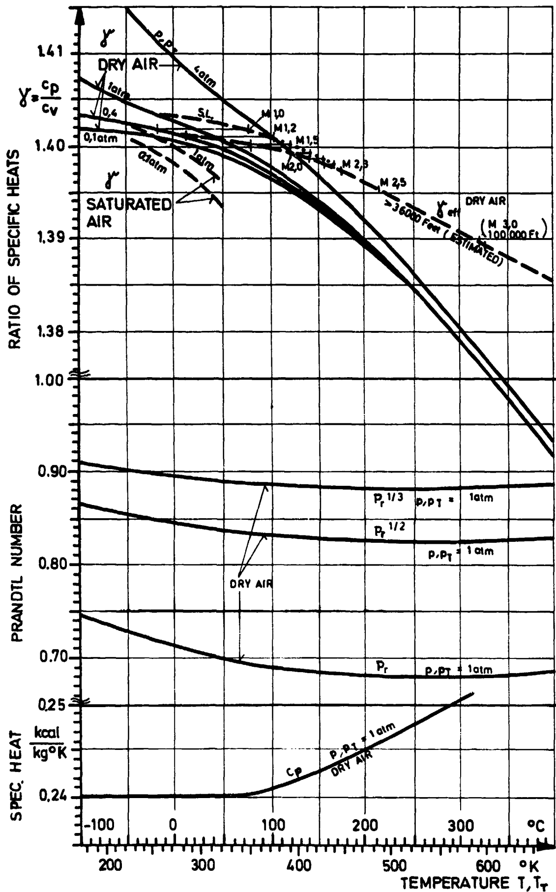
Fig.62(a) Variations of gas properties vs temperature
