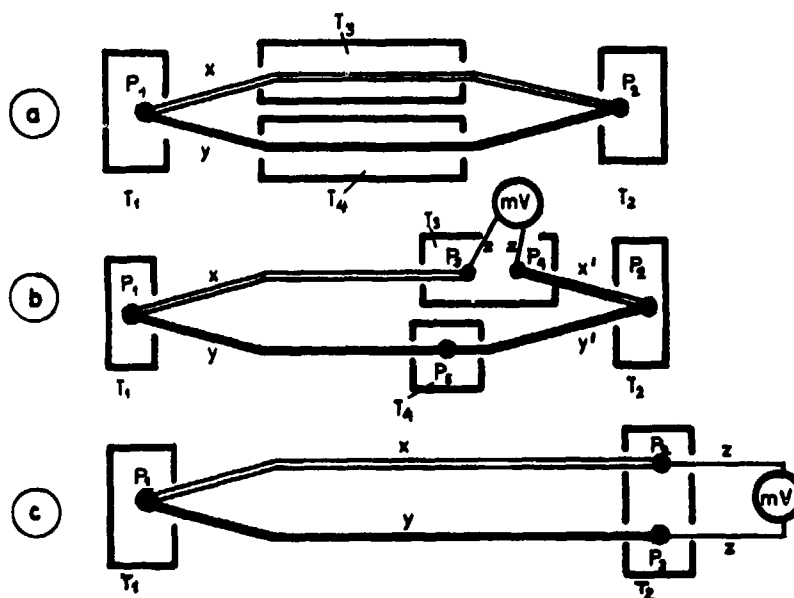
Fig. 42 Circuits with thermocouples
