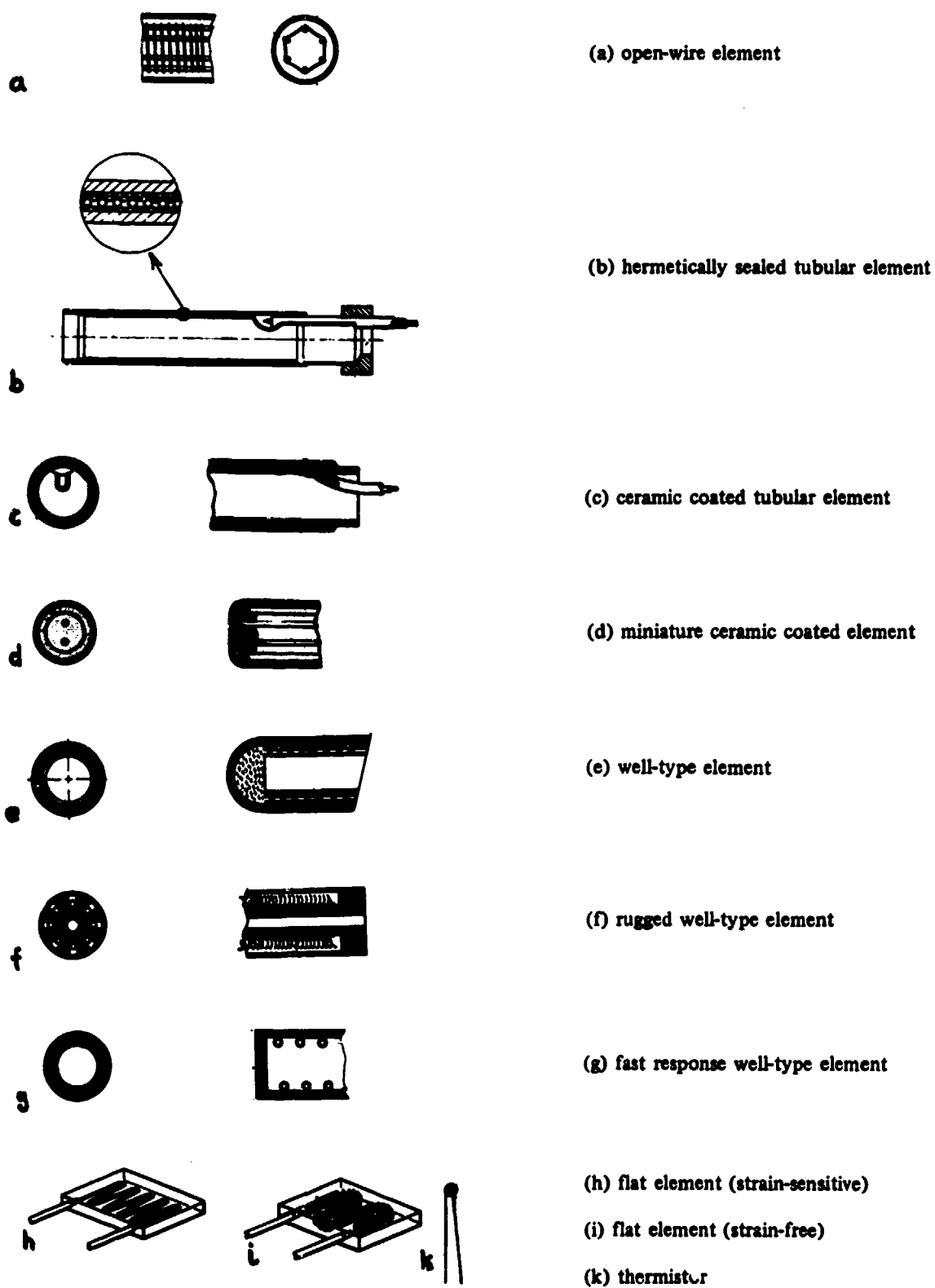
Fig.9 Construction of resistance probes
