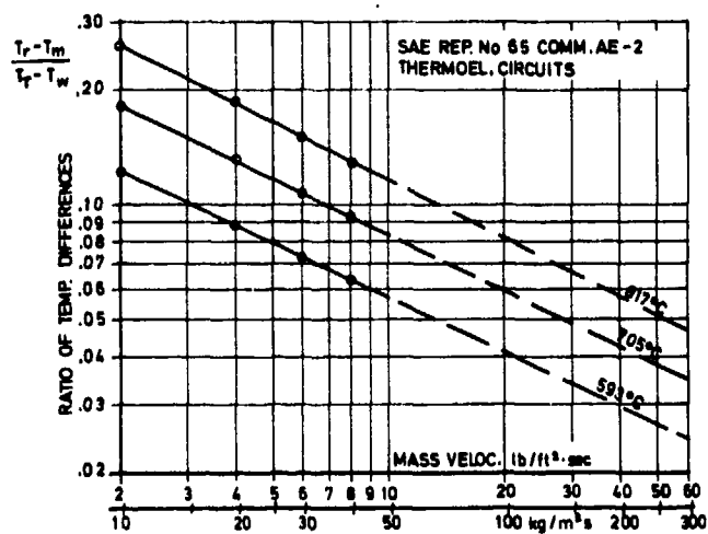
Fig.72 Radiation and conduction correction factors vs flow rate for a typical tailpipe temperature sensor with bare wire loop junction (16 Ga round wire)
