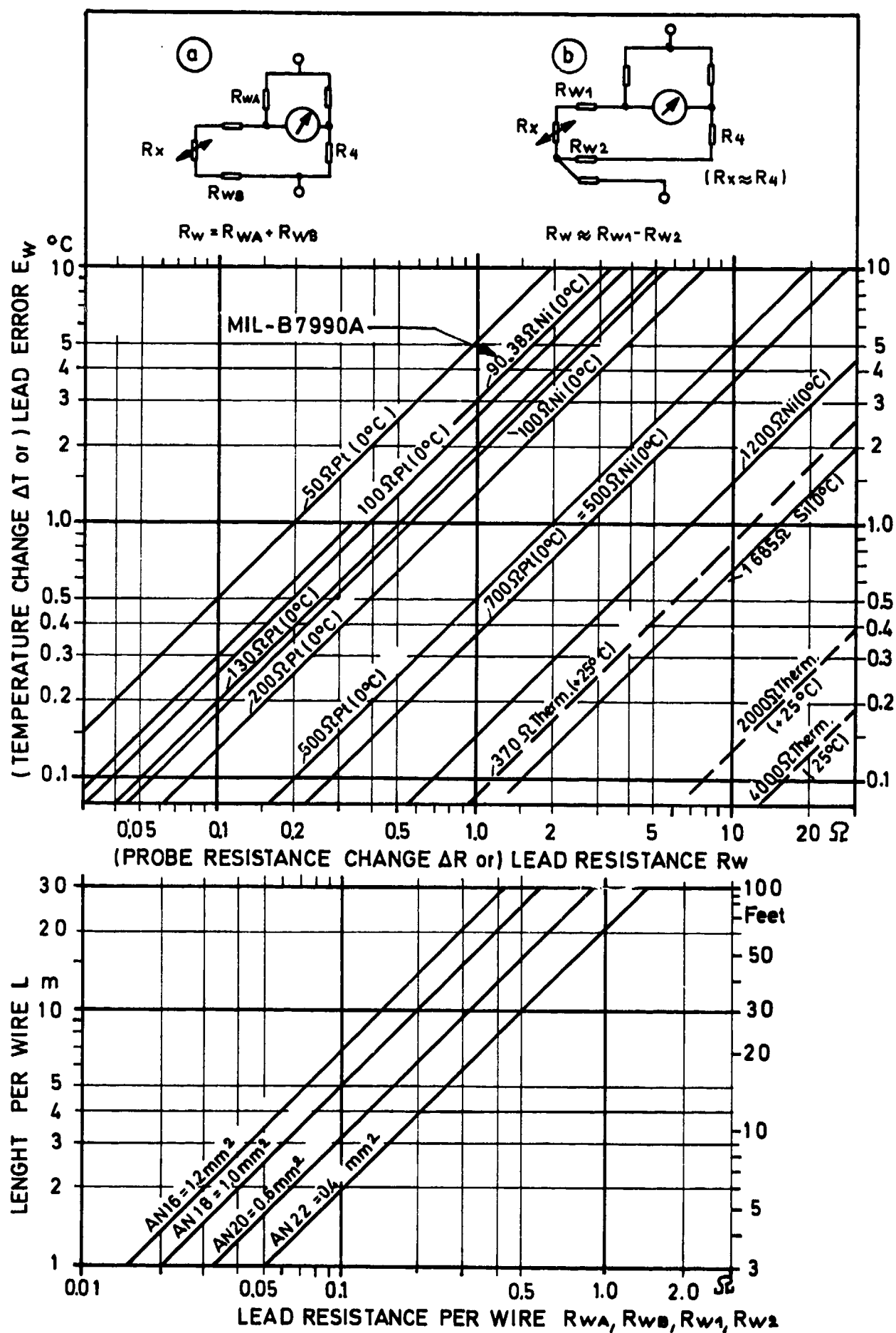
Fig.89 Electric lead error of temperature probes
