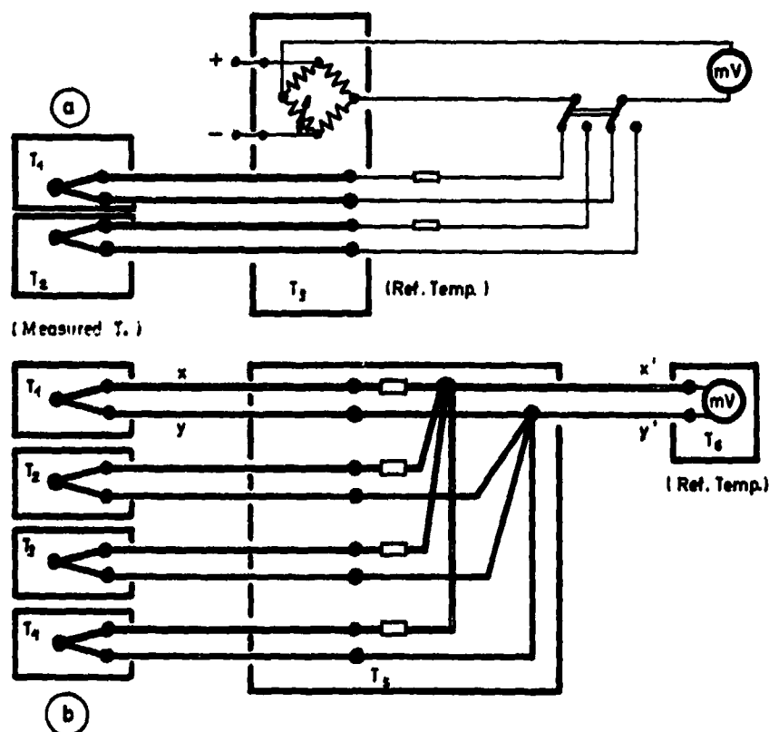
(a) measurement on different positions (b) measurement of mean temperature
