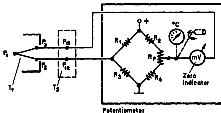
Fig.48 Thermocouple with potentiometer circuit
