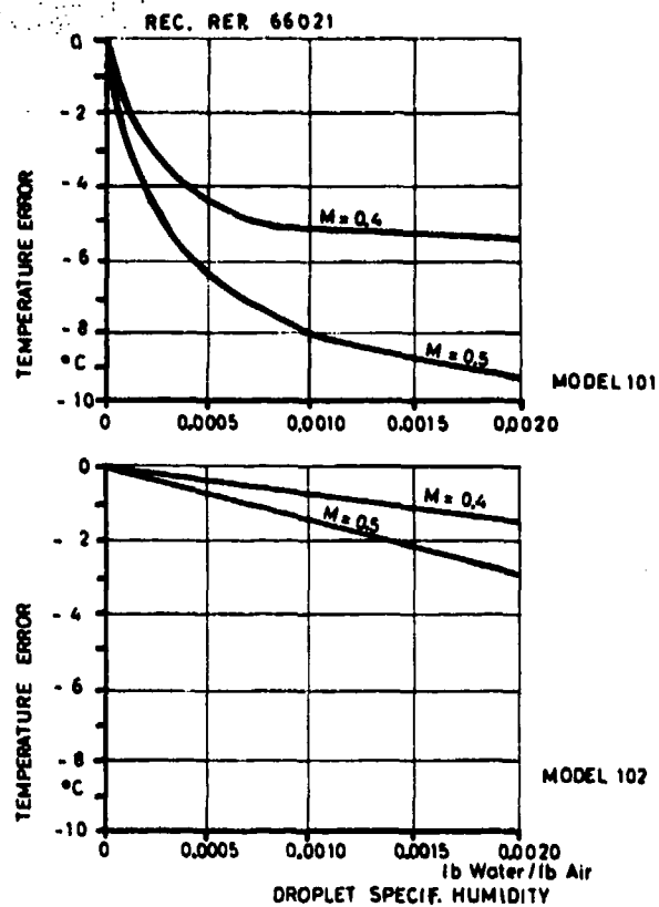
Fig.70 Typical errors due to water droplets
