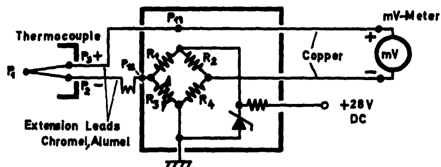
Fig.46 Wiring diagram – thermocouple thermometer with compensating bridge circuit
