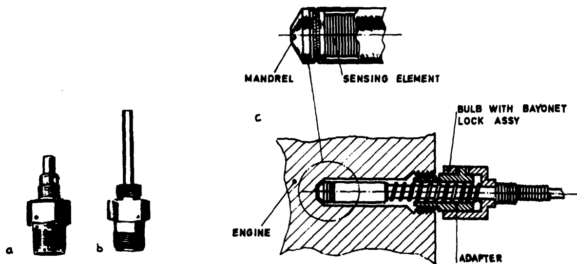
(a,b) fixed well-type probes (c) spring-loaded type with bayonet lock assembly
