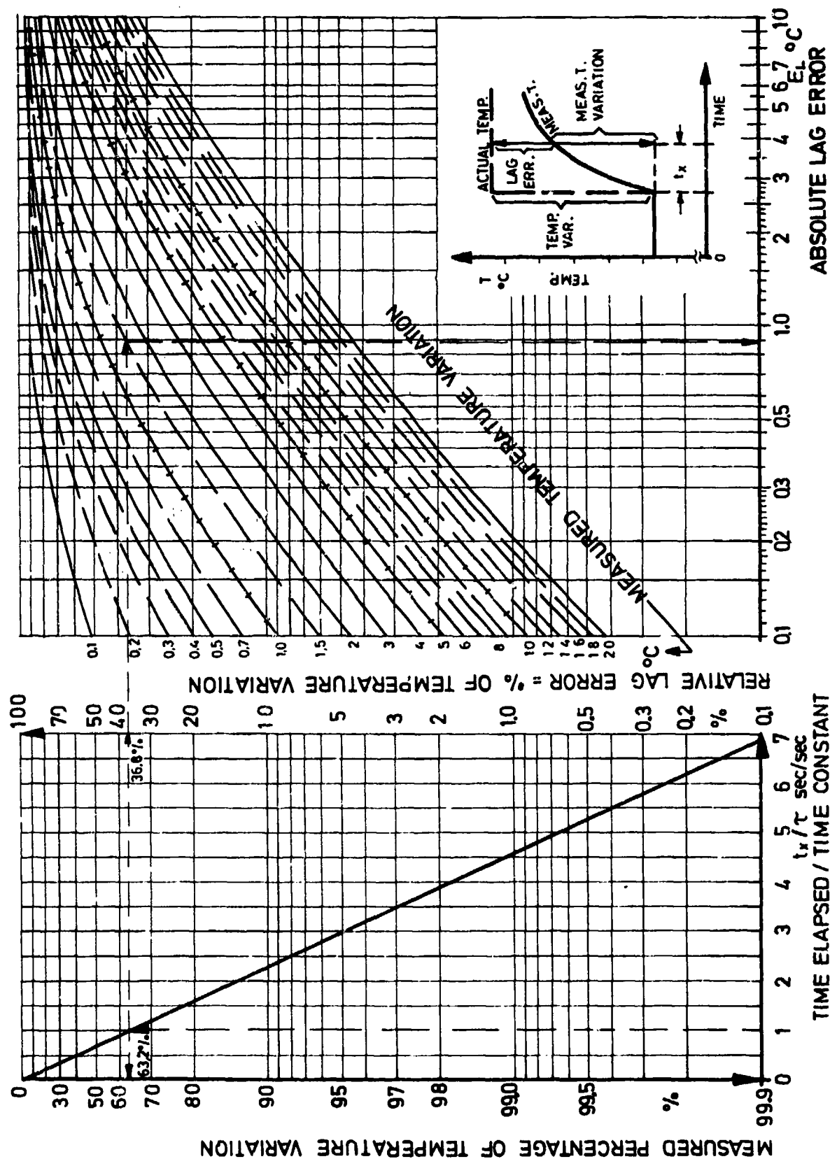
Fig.8.4 Temperature lag error as a function of time elapsed and measured variation in temperature
