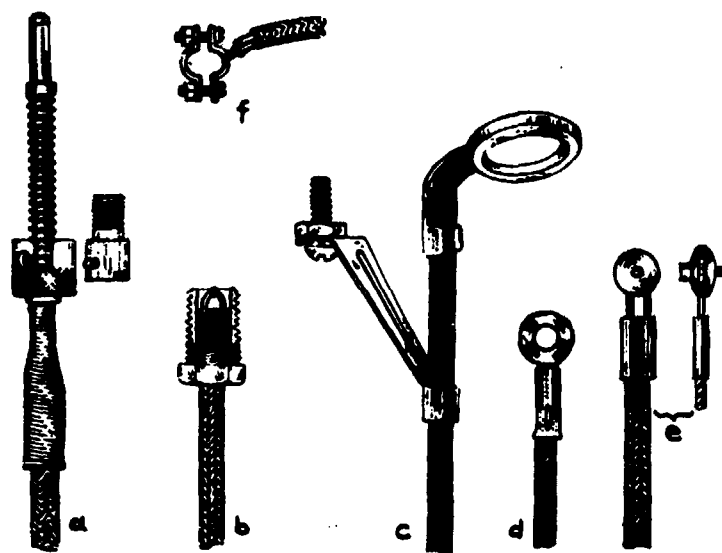
Fig. 40 Special TAT probe with thermocouple
