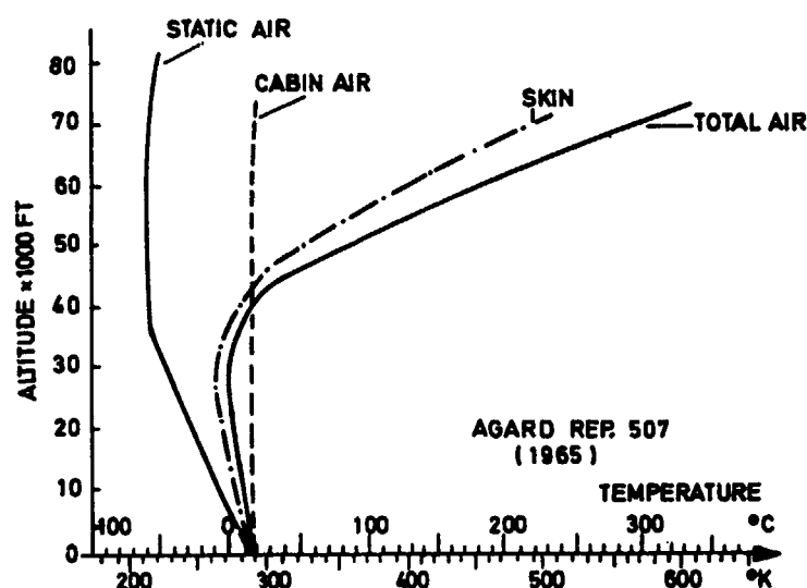
Fig.2 Environmental temperatures of supersonic aircraft
