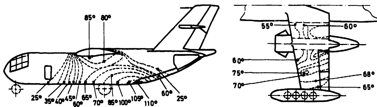
Fig.98(b) Typical distribution of skin temperatures at vertical take-off
