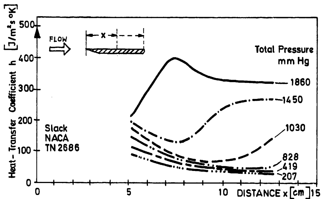
Fig.51 Heat transfer coefficient vs distance and pressure
