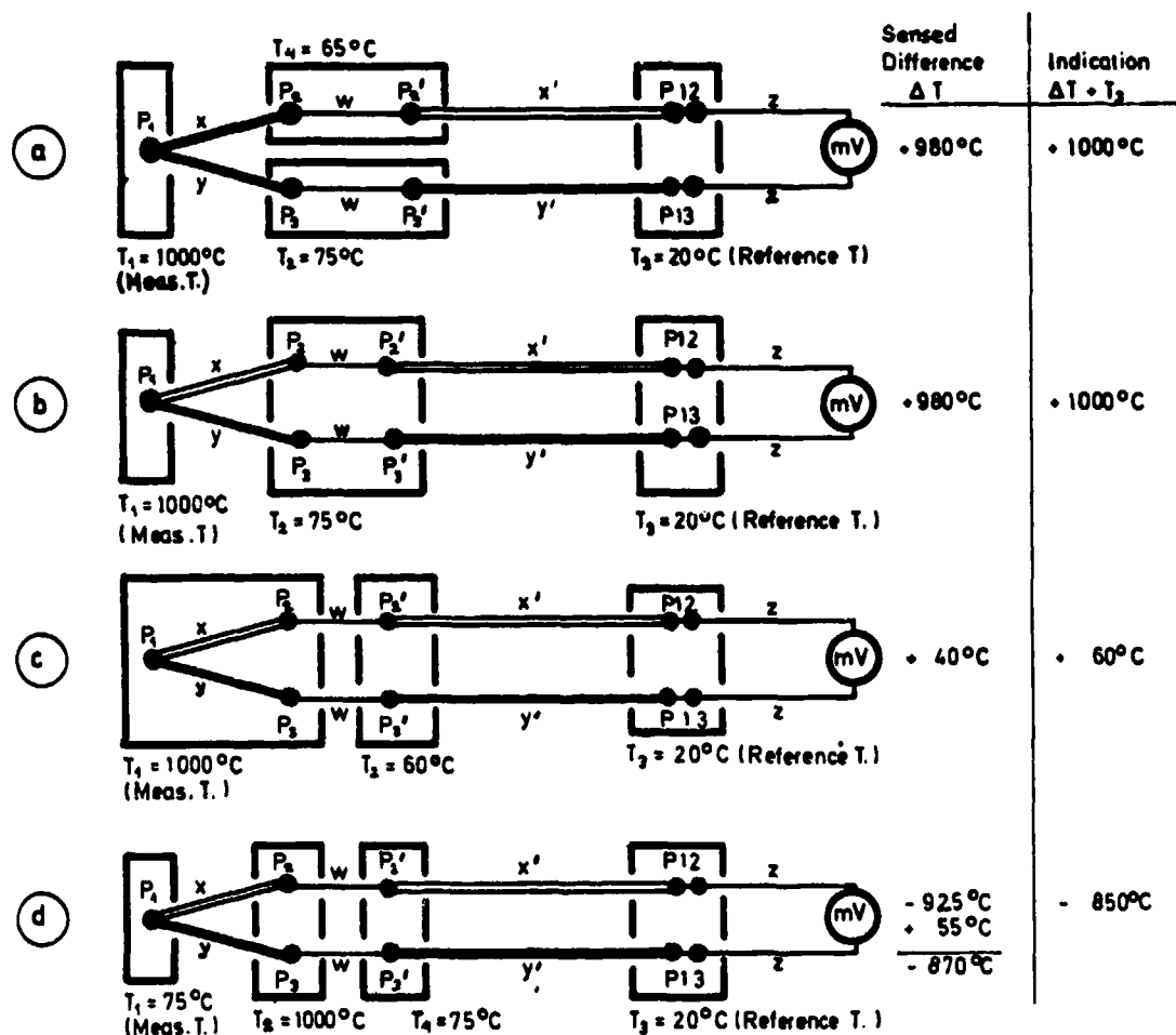
Fig.43 Temperature indications with different locations of the gradient
