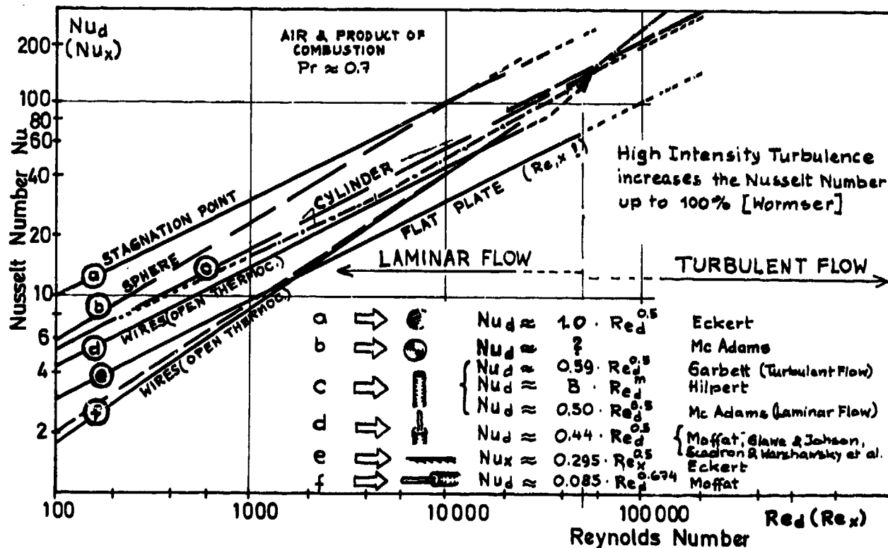
Fig.52 Nusselt number as a function of Reynolds number and shape of probe
