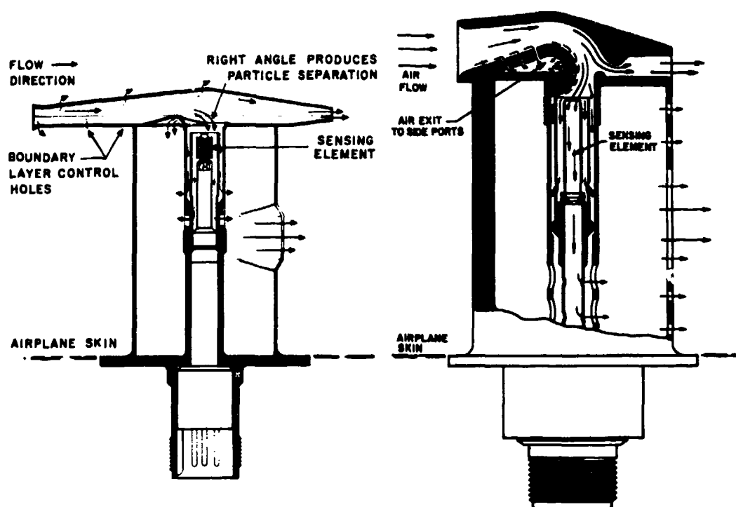
Fig. 18 Internal construction of TAT probes with air flow deflection in front of the elements
