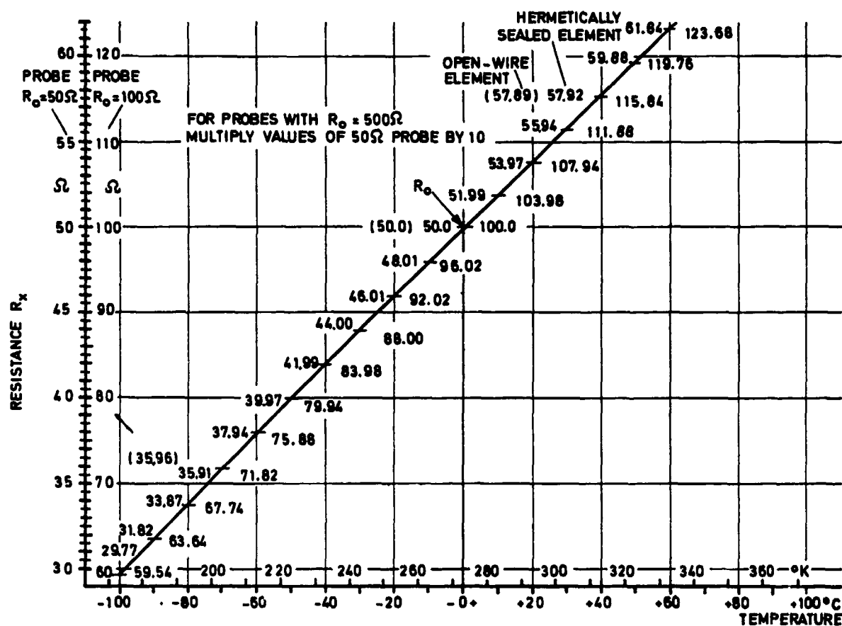
Fig.5(a) Resistance-temperature relationship of platinum elements MIL-P-28726 range -100 to +60^\circ\text{C}
