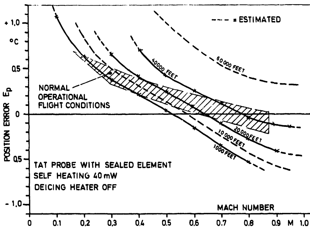
Fig.100 Position error of a TAT-probe with ratiometer (theoretical values)
