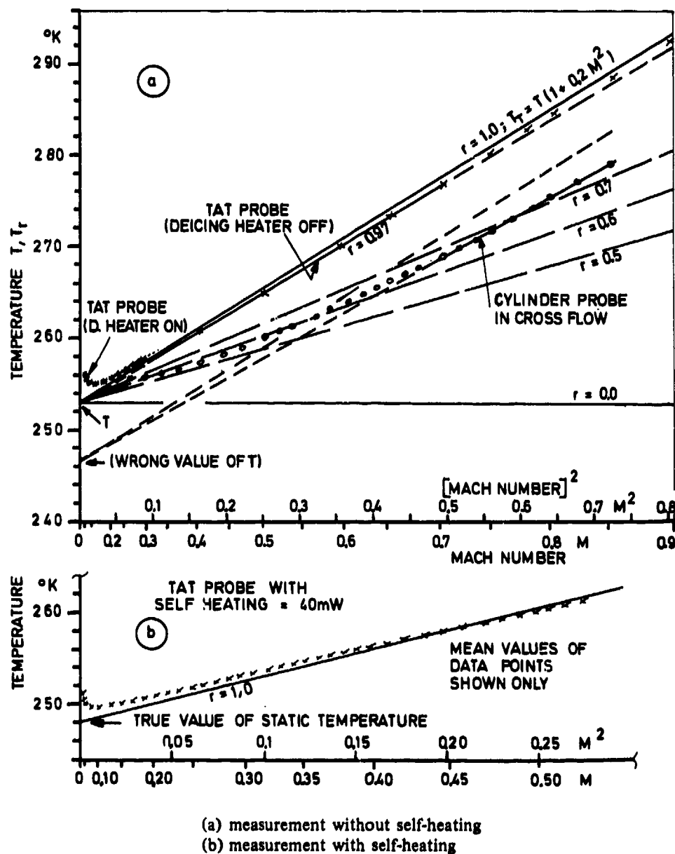
Fig.102 Evaluation of the recovery factor
