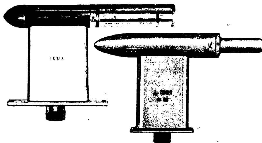
Fig.16 Total temperature probes
