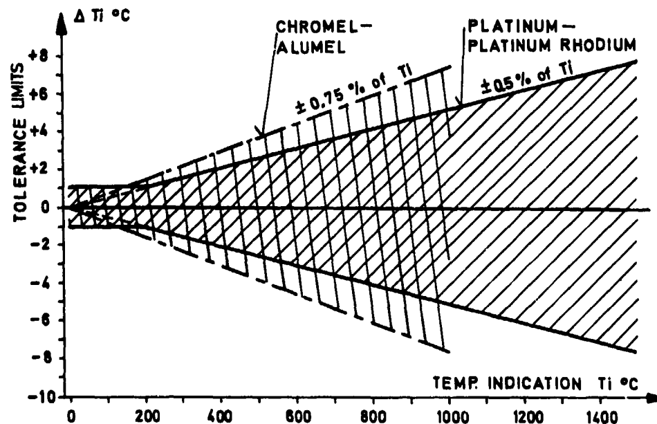
Fig. 88 Typical tolerances (calibration error) of thermocouples
