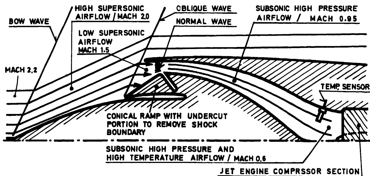
Fig.65 Compressor inlet temperature measurement (typical flow conditions at flight Mach number 2.0)
