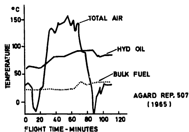
Fig.3 Temperatures vs time for supersonic flight
