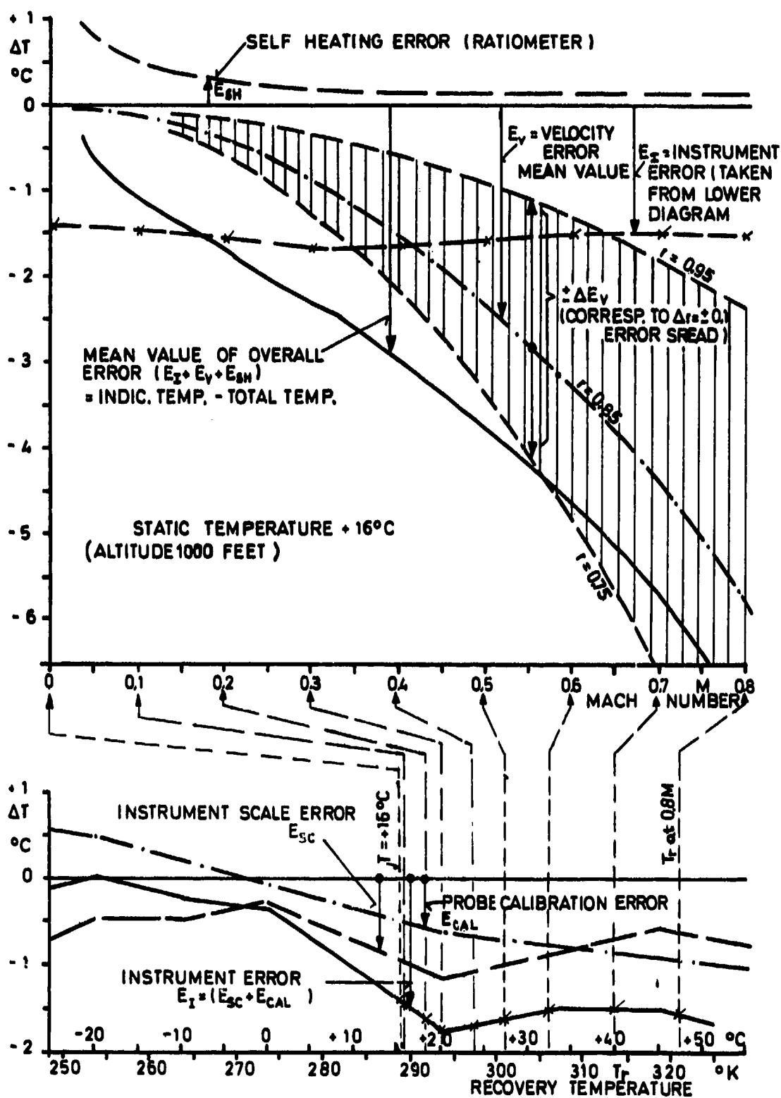
Fig.106 Temperature error components of simple probe (120 \Omega , Ni) with ratiometer indicator
