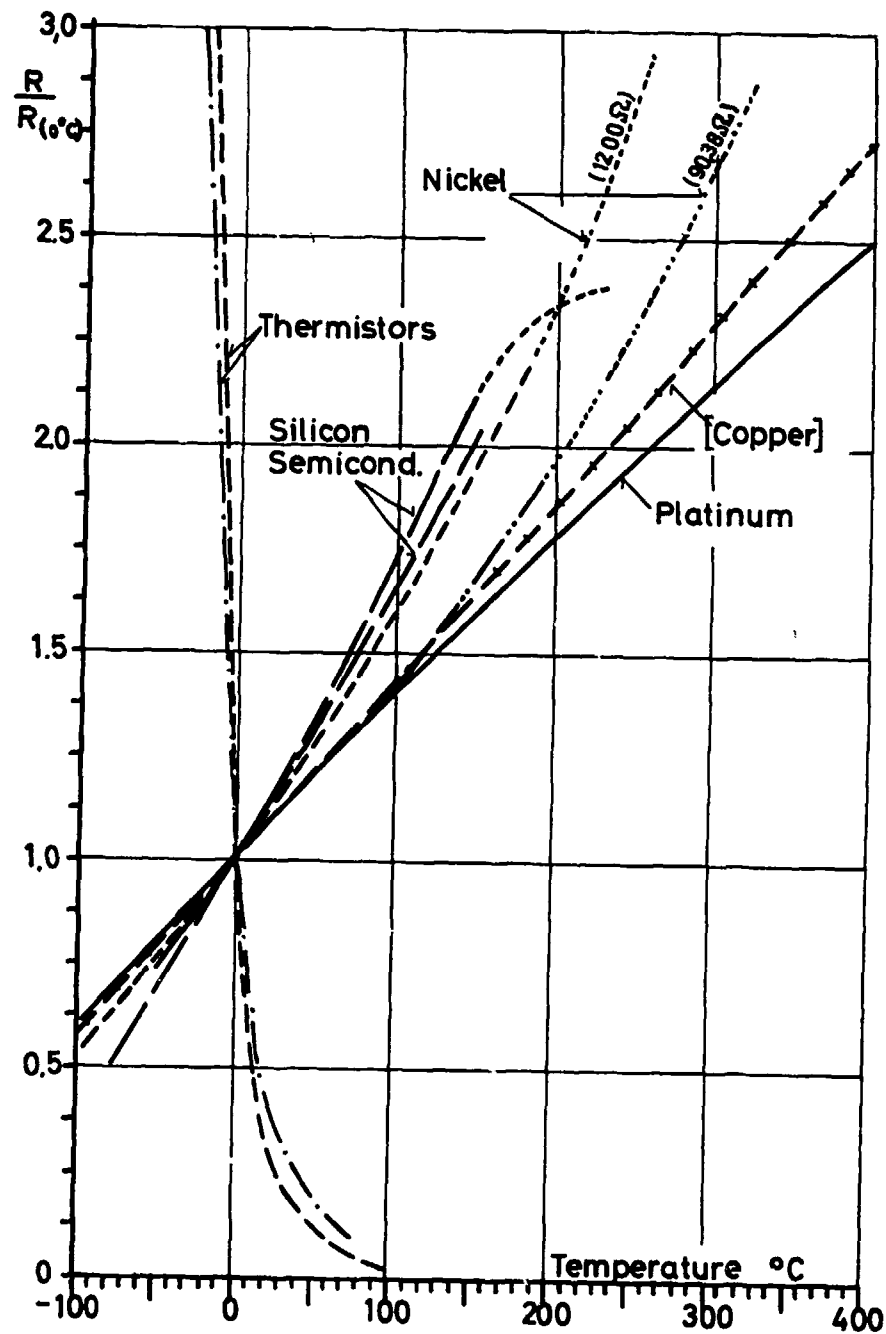
Fig.4 Resistance-temperature relationship of some temperature elements
