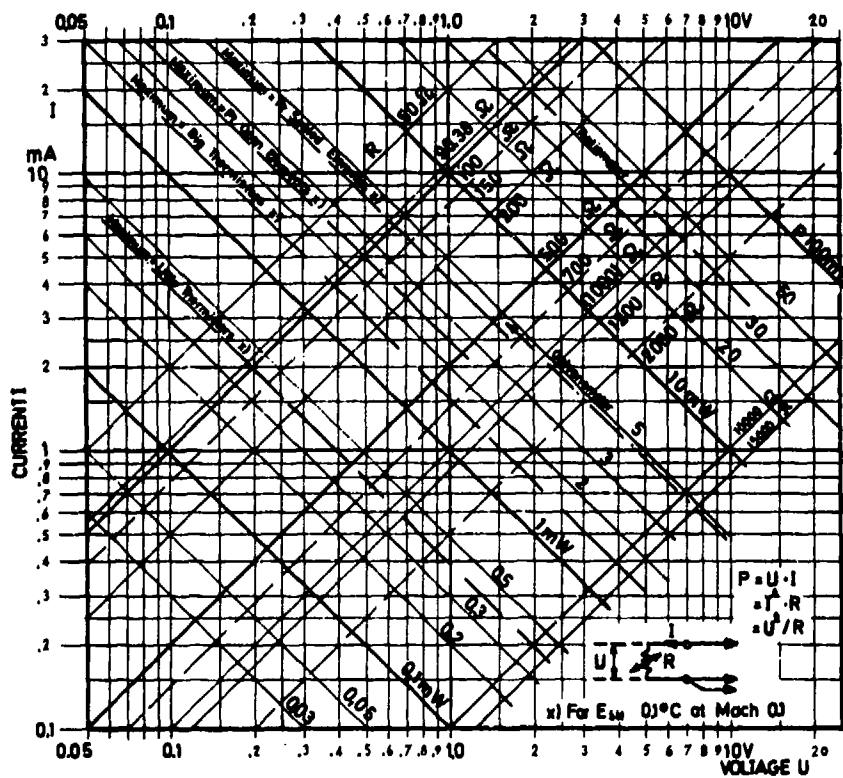
Fig.74 Self-heating power in temperature probes
