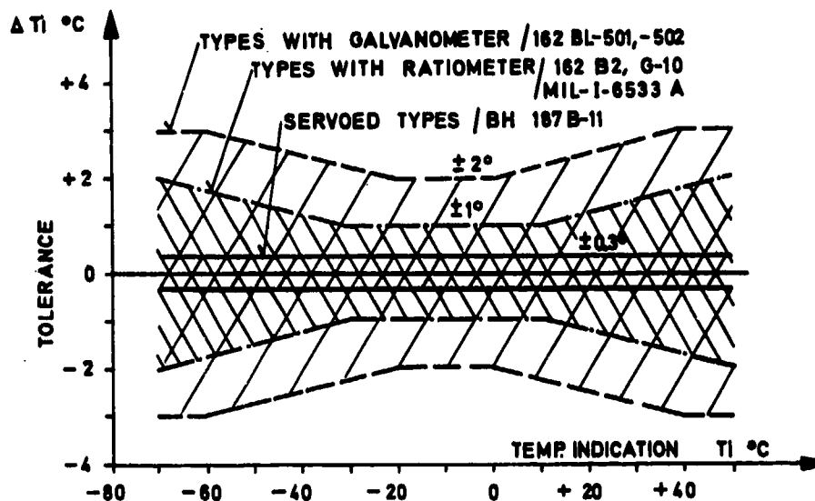
Fig.90(b) Typical tolerances (scale error) of some indicators (without probe)
