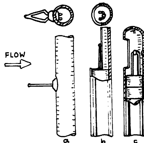
Fig. 39 Simple TAT probes with thermocouples
