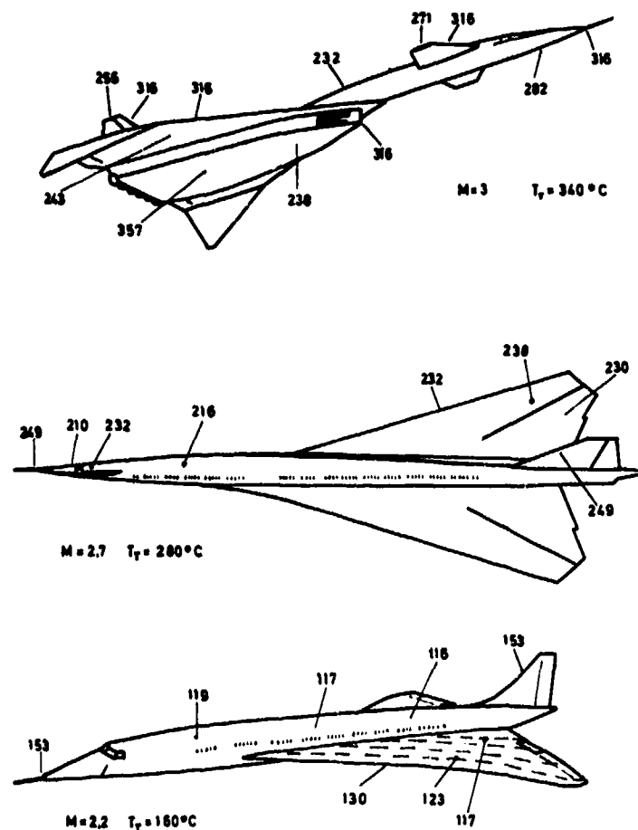
Fig.97 Skin temperatures of supersonic aircraft ( ^\circ\text{C} )
