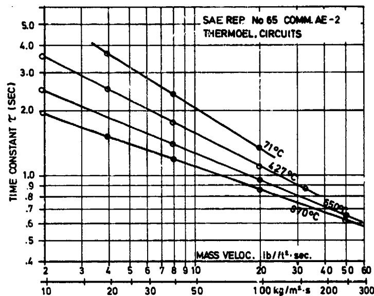
Fig.82 Time constant vs. flow rate for a typical tailpipe temperature sensor with bare wire loop junction (16 Ga. round wire)
