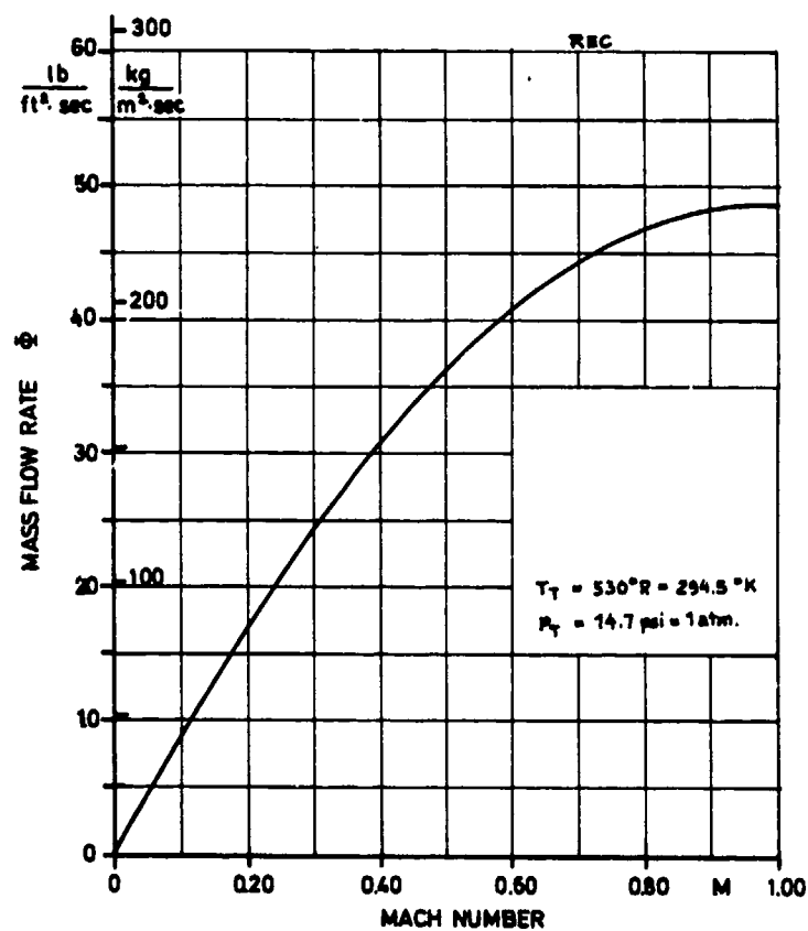
Fig.62(c) Variation of mass flow rate with Mach number for constant T_T and P_T
