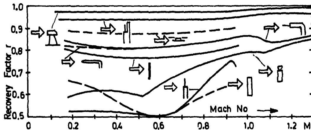
Fig.55 Recovery factors of different probes vs Mach number (for typical mounting positions)
