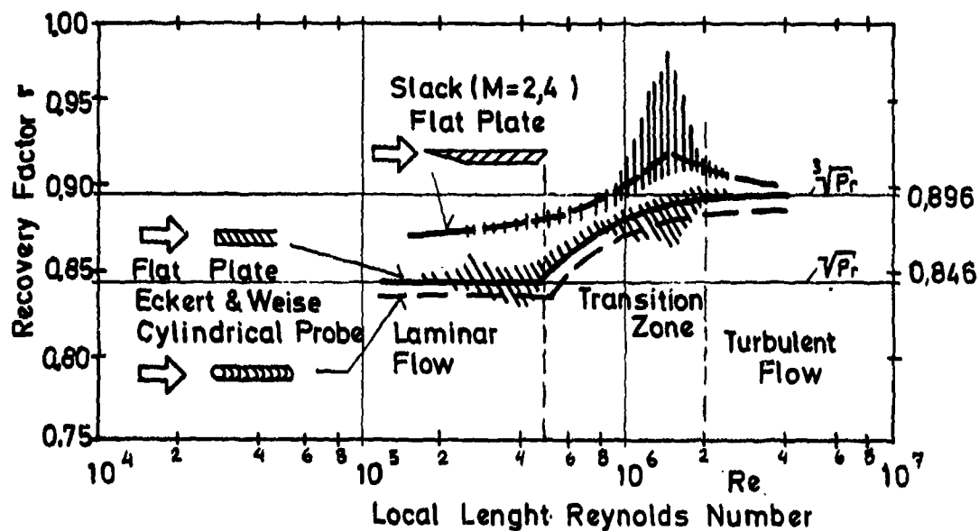
Fig.53 Recovery factor as a function of Reynolds number and shape of probe
