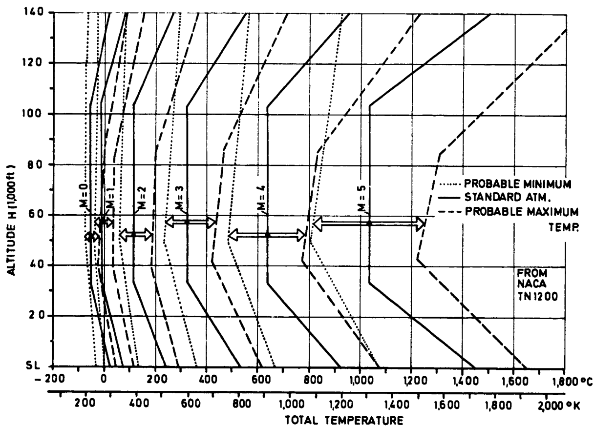
Fig.61 Total temperature as a function of altitude and Mach number
