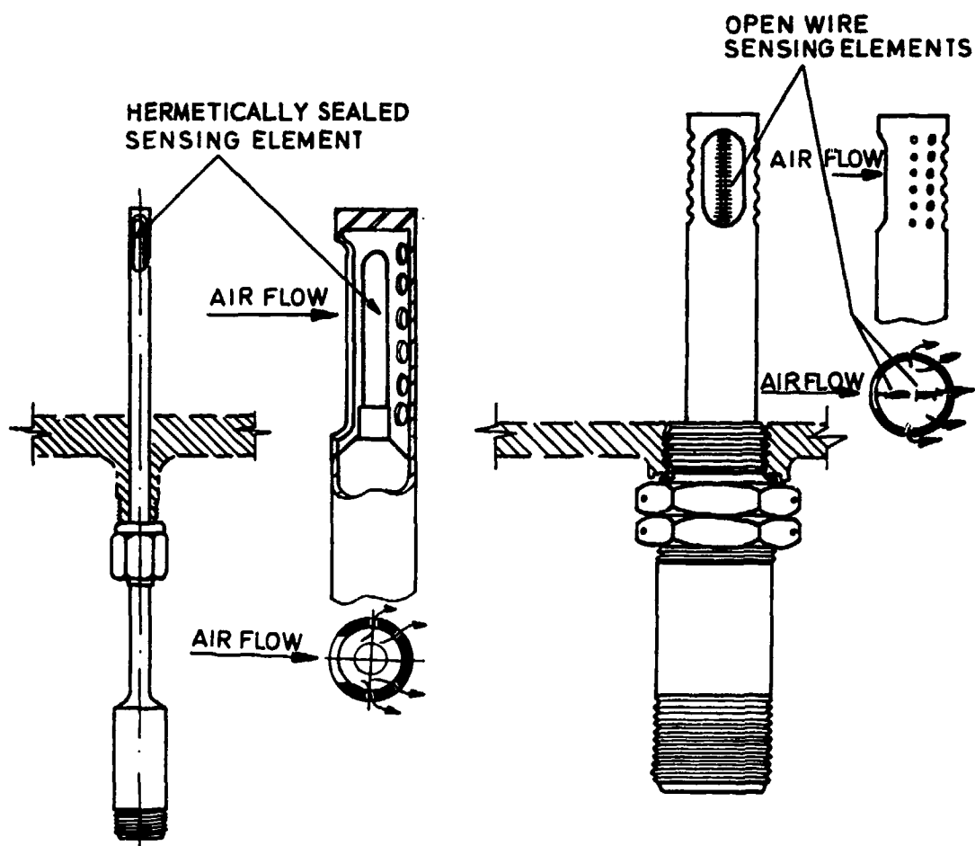
Fig.20 Internal construction of simple TAT probes for compressor inlet temperature measurements
