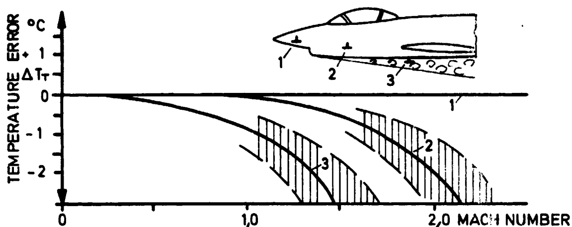
Fig.63 Typical probe location errors (estimated)
