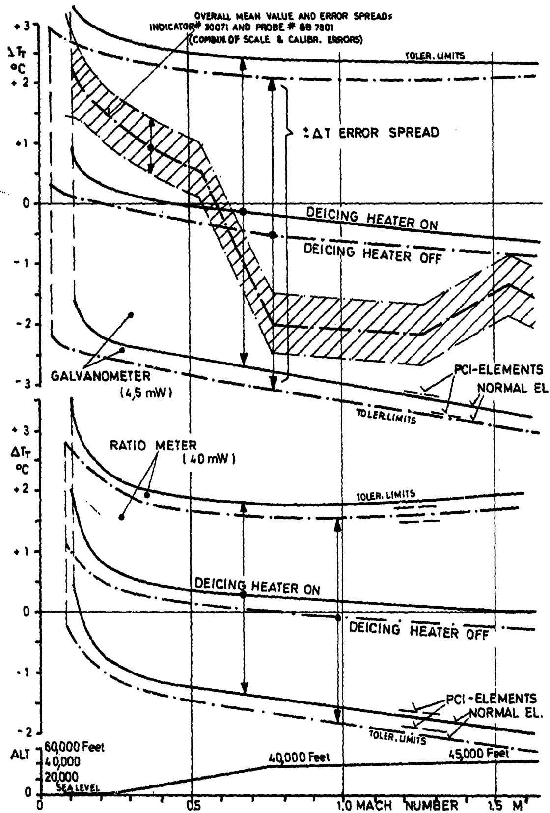
Fig.109 Overall temperature error of a TAT-probe with ratiometer or galvanometer
