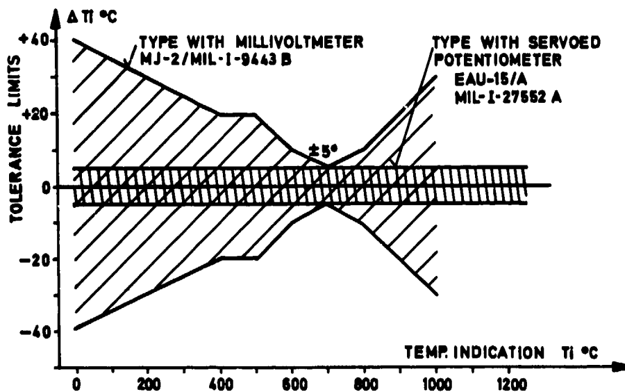
Fig.91 Typical tolerances (instrument error) of indicators (without probe)
