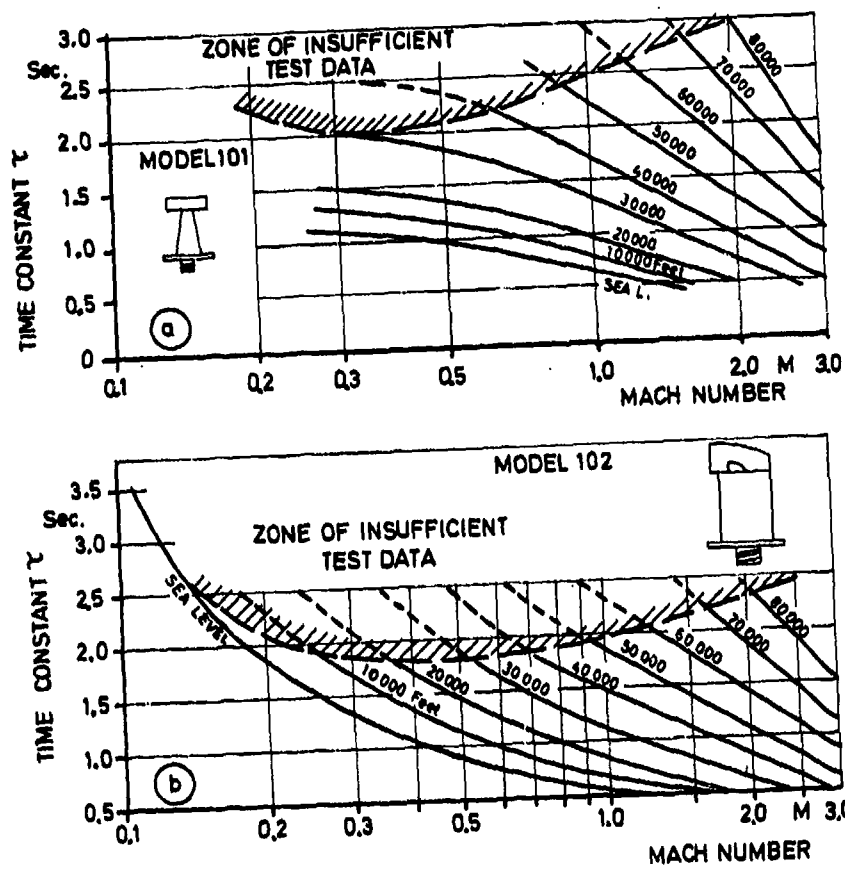
Fig.80(a,b) Time constant of some probes
