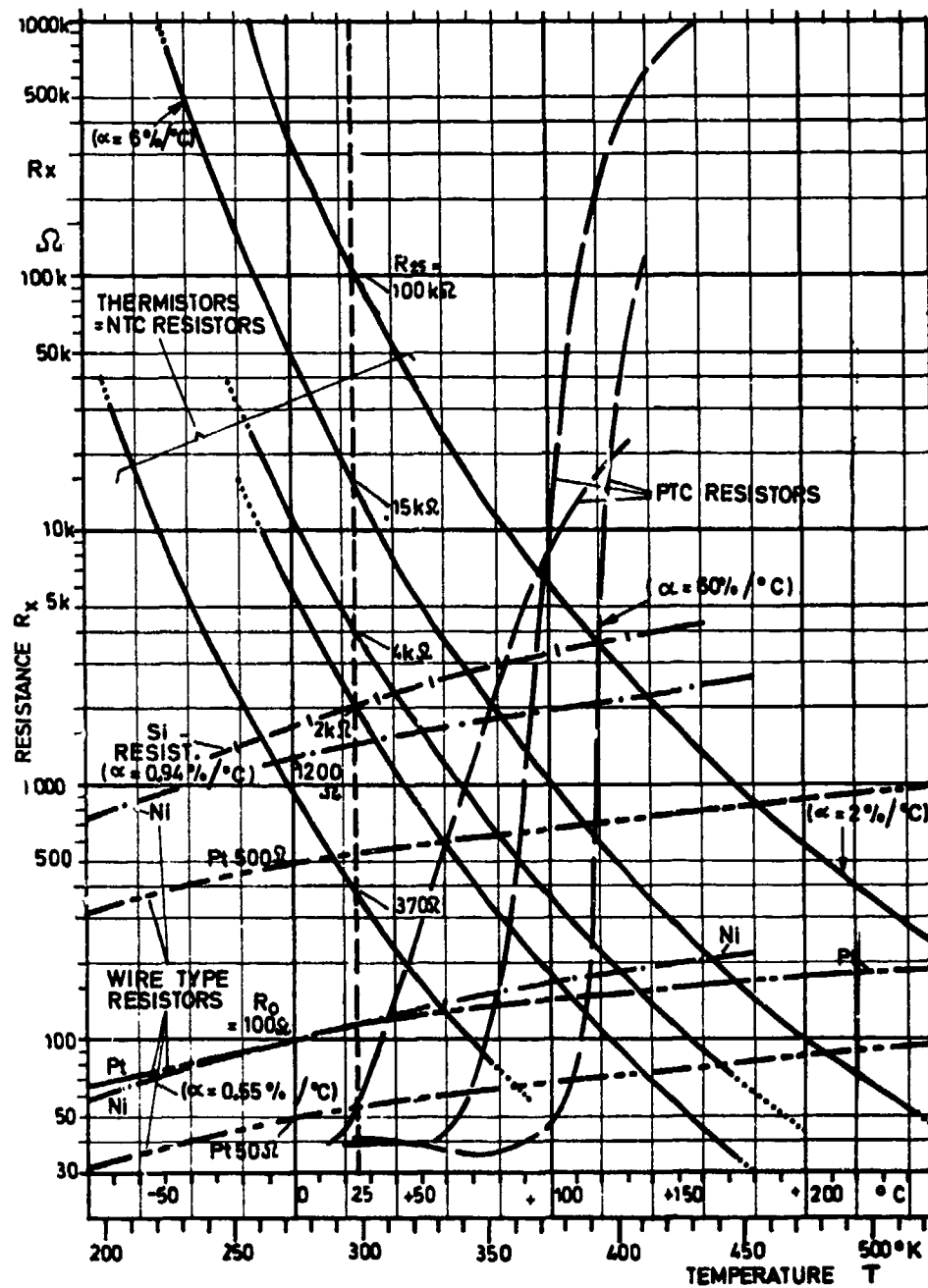
Fig. 7 Characteristics of resistance elements, temperature vs resistance
