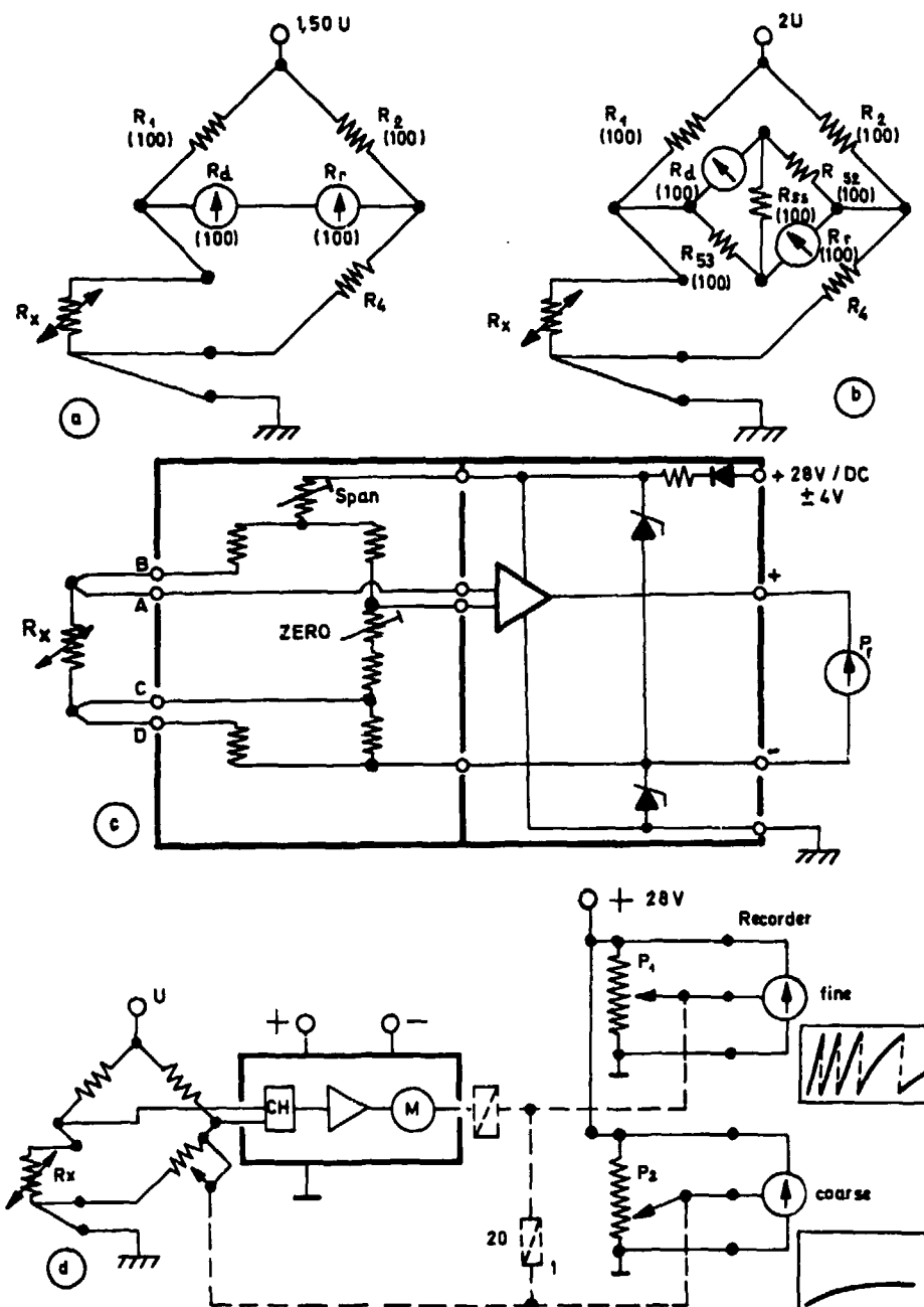
(a,b) full bridge circuits (c) signal conditioner (d) servoed bridge
