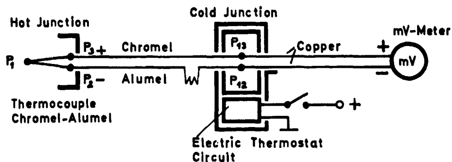
Fig.45 Wiring diagram -- thermocouple thermometer with thermostat as reference point
