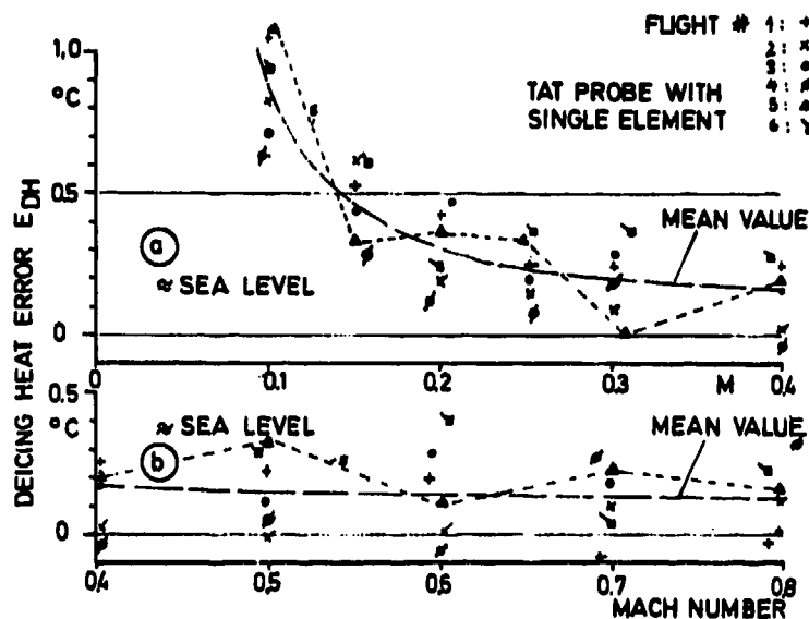
Fig.101 Deicing heat error of a TAT-probe (typical test results)
