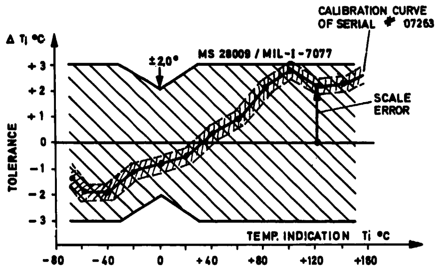
Fig.90(a) Typical tolerances of resistance thermometer indicator at room temperature (ratiometer without probe)
