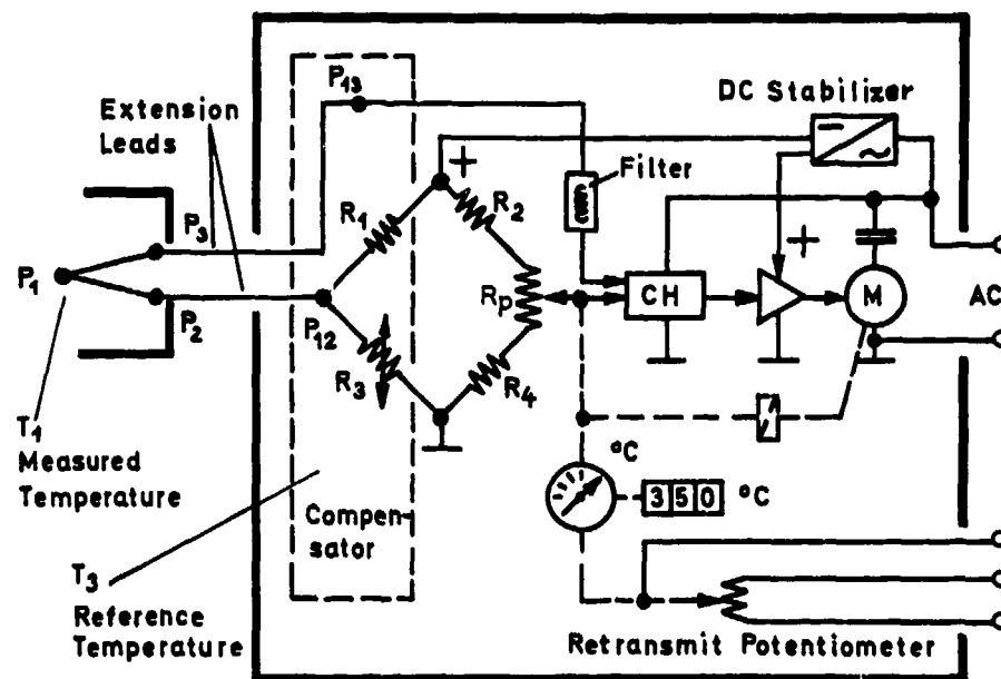
Fig.49 Thermocouple with servo temperature indicator
