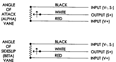
ELECTRICAL SCHEMATIC
