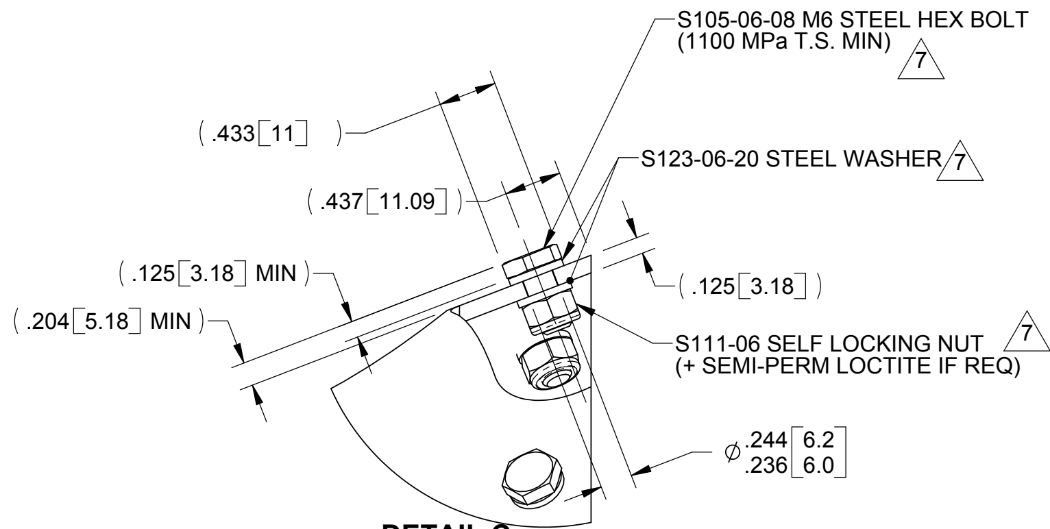
DETAIL C SCALE 1 : 1 (15 PLS)
